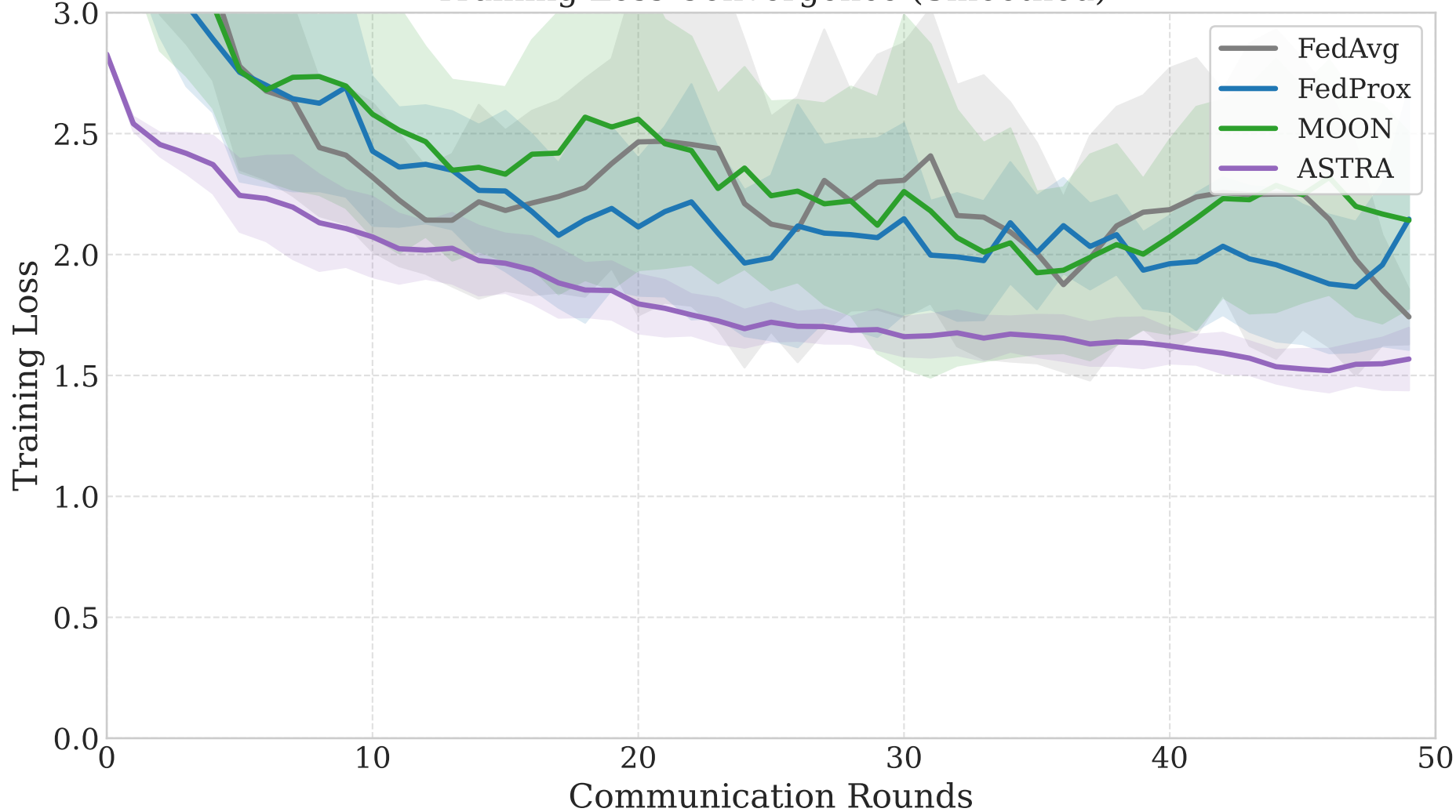
Training Loss Convergence (Smoothed)
