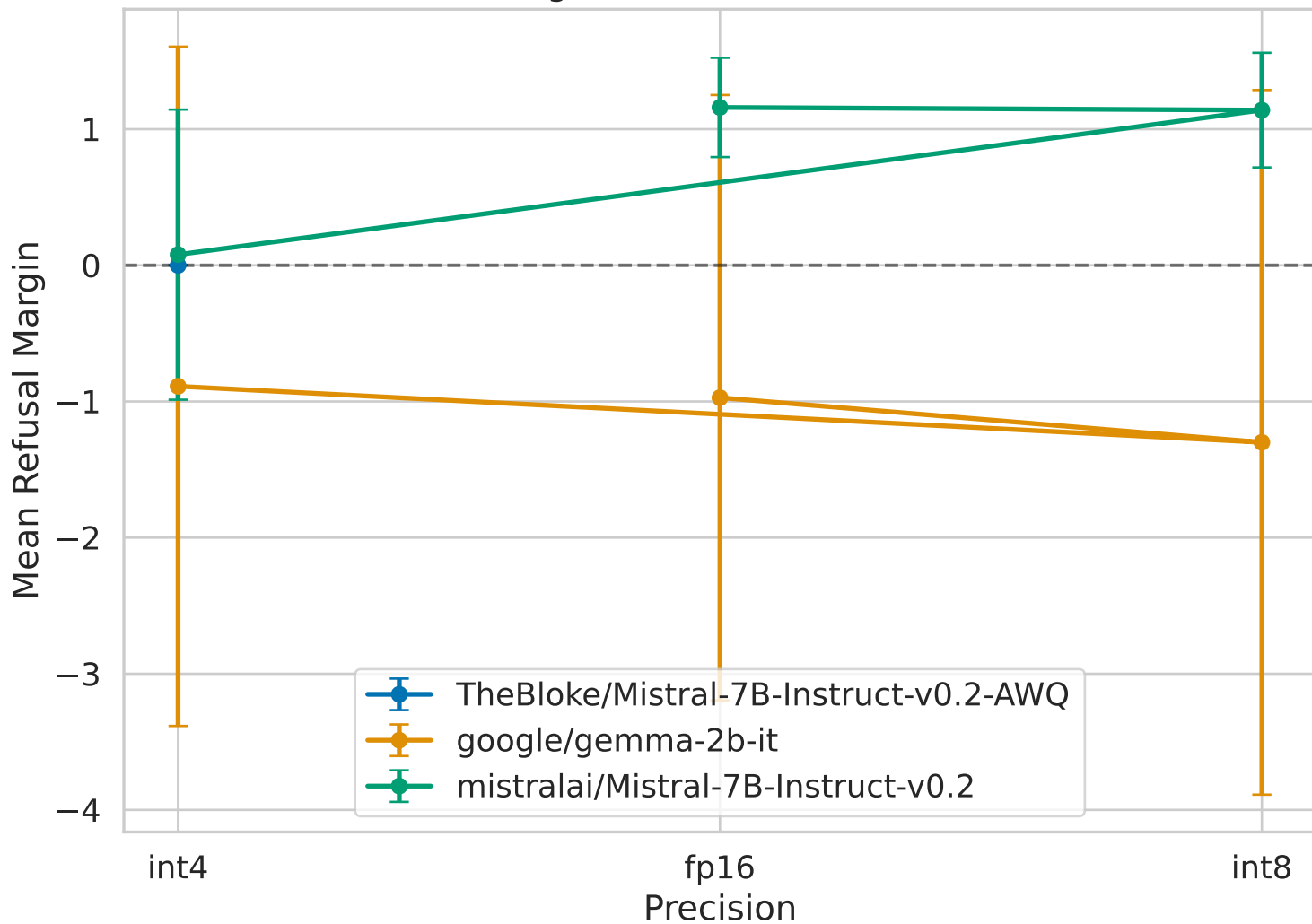
Refusal Margin Robustness Across Precision
