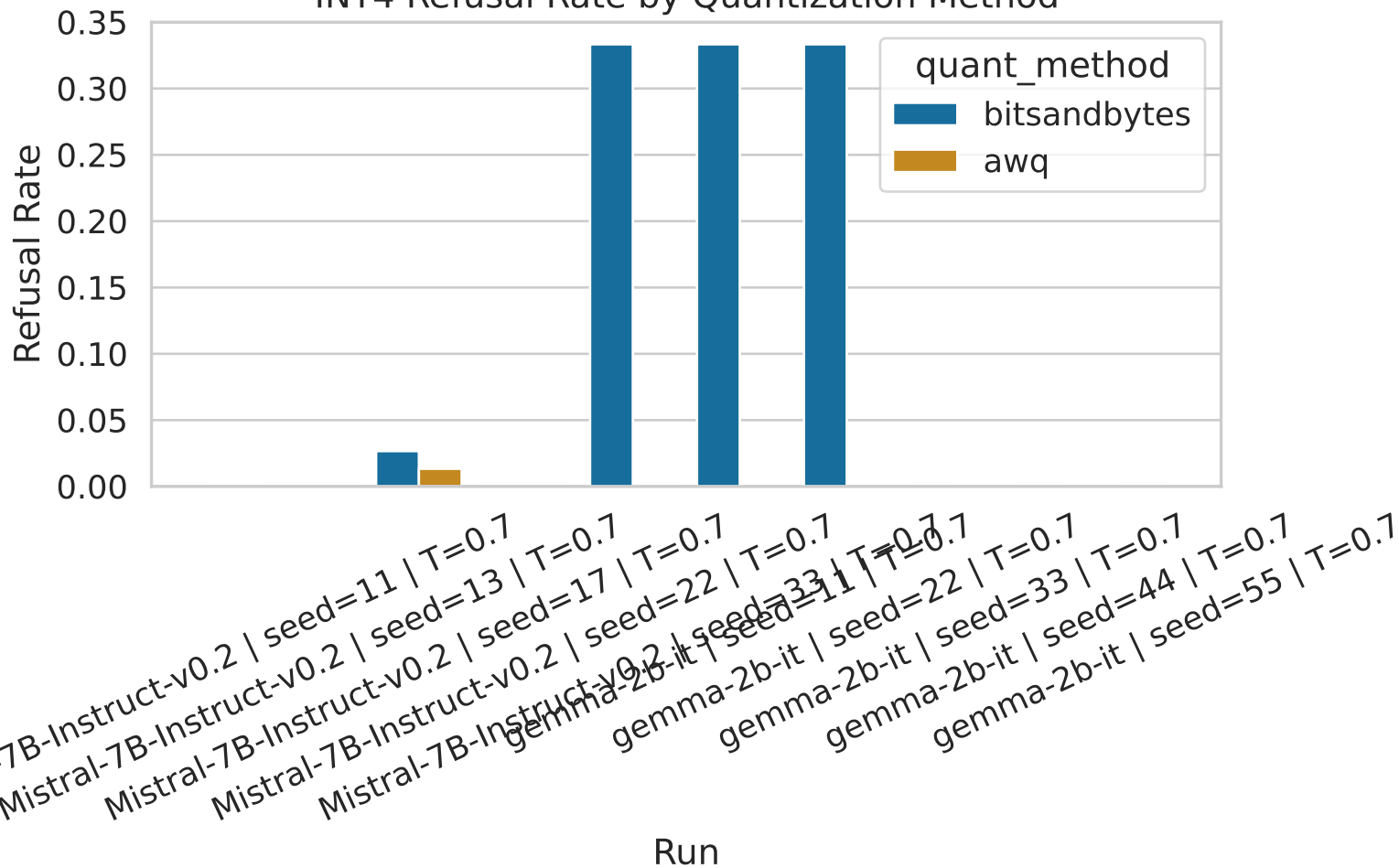
INT4 Refusal Rate by Quantization Method
