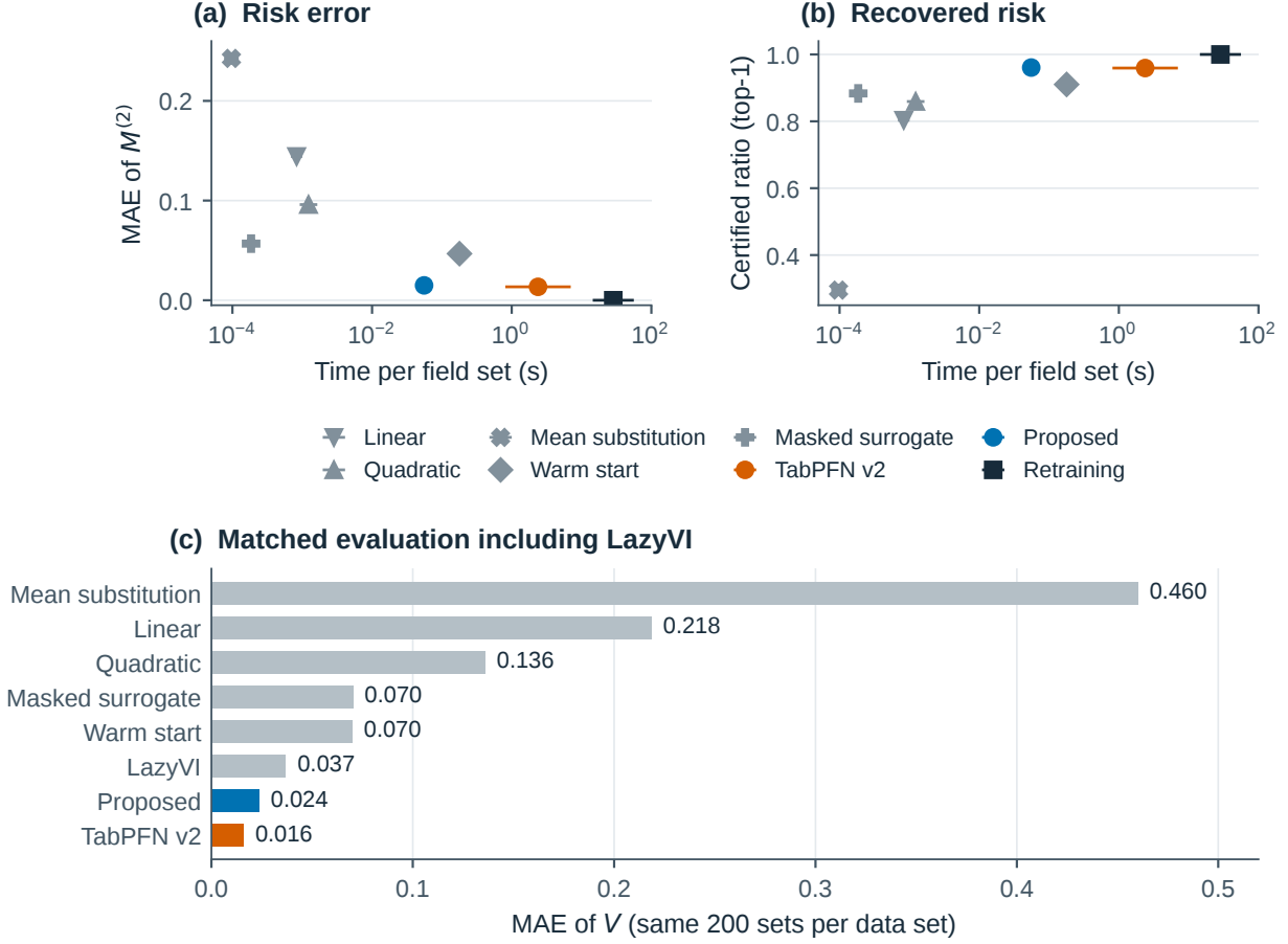
Figure 10: Comparison with other estimators over ten targets. (a) Error of M^{(2)} and (b) certified top-1 ratio against the time per field set (all targets of a data set; bars: range over data sets); retraining defines the ground truth. (c) Error of V on the same 200 sets per data set for every method, including LazyVI, which was too slow to run on all sets.
