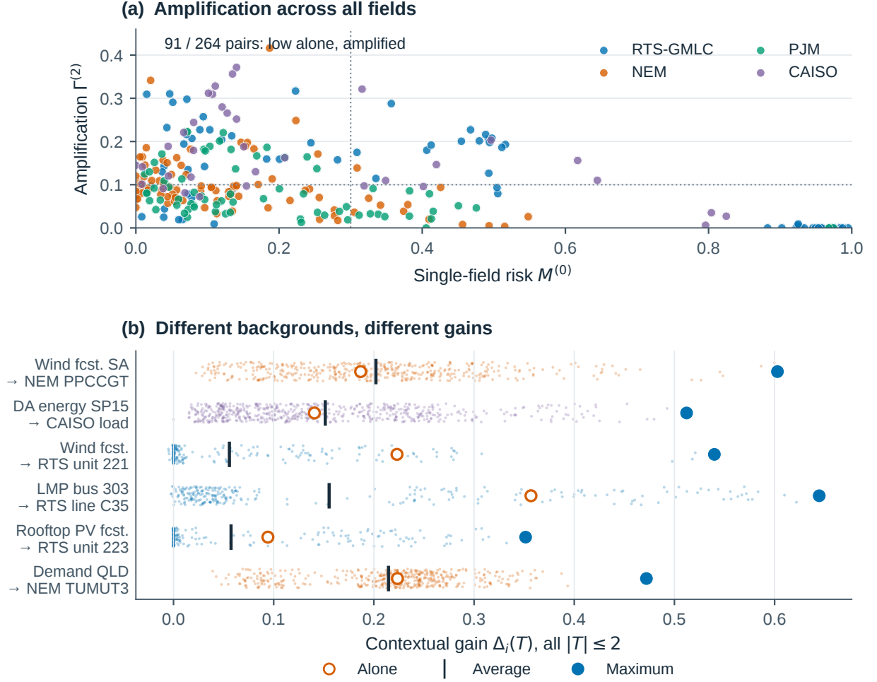
Figure 5: Background amplification over ten targets. (a) Single-field risk versus amplification \Gamma^{(2)} for every field–target pair. (b) Contextual gains of the most amplified field of six targets over all backgrounds of at most two fields, with the single-field value, the average over backgrounds and the maximum.
