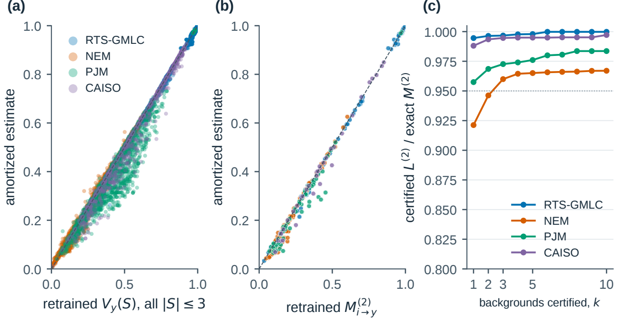
Figure 9: Amortized estimates against retrained ground truth. (a) \hat{V}_y(S) for sets of size \leq 3 (random subsample). (b) \hat{M}^{(2)} for every field and target. (c) Certified lower bound over exact M^{(2)} when the top- k scanned backgrounds per field are retrained.
