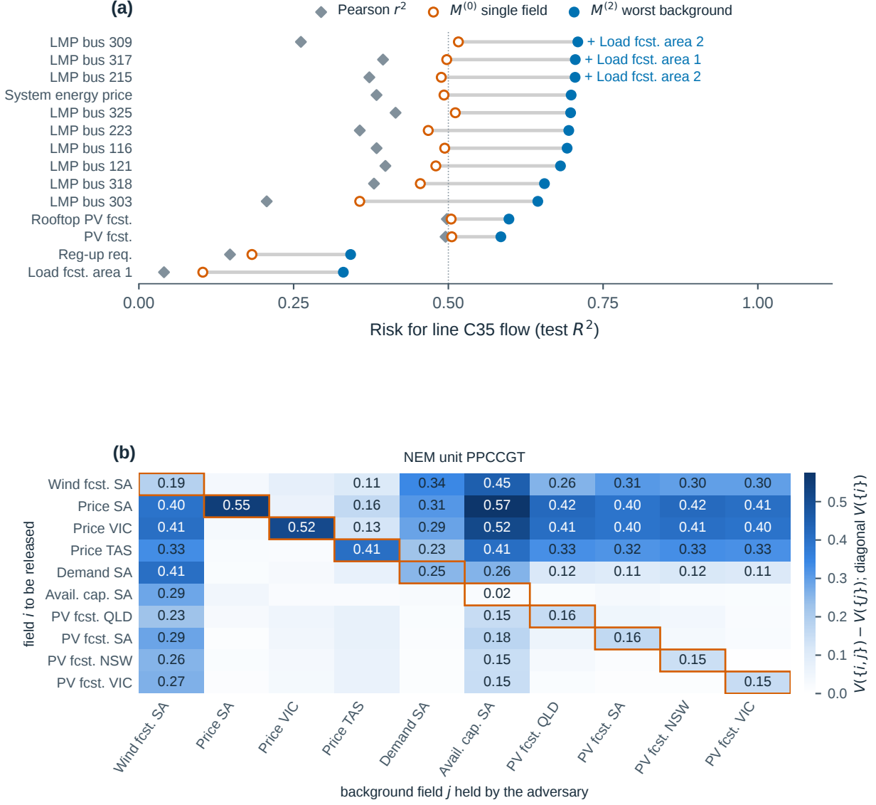
Figure 7: (a) Field profile for the hourly flow on RTS line C35 (14 fields with the largest M^{(2)} ): Pearson r^2 , single-field risk and worst-background risk, with the witness background for the three riskiest fields. (b) Gain matrix for NEM unit PPCCGT: entry (i, j) is V(\{i, j\}) - V(\{j\}) , the diagonal is V(\{i\}) ; values below 0.10 are not printed.
