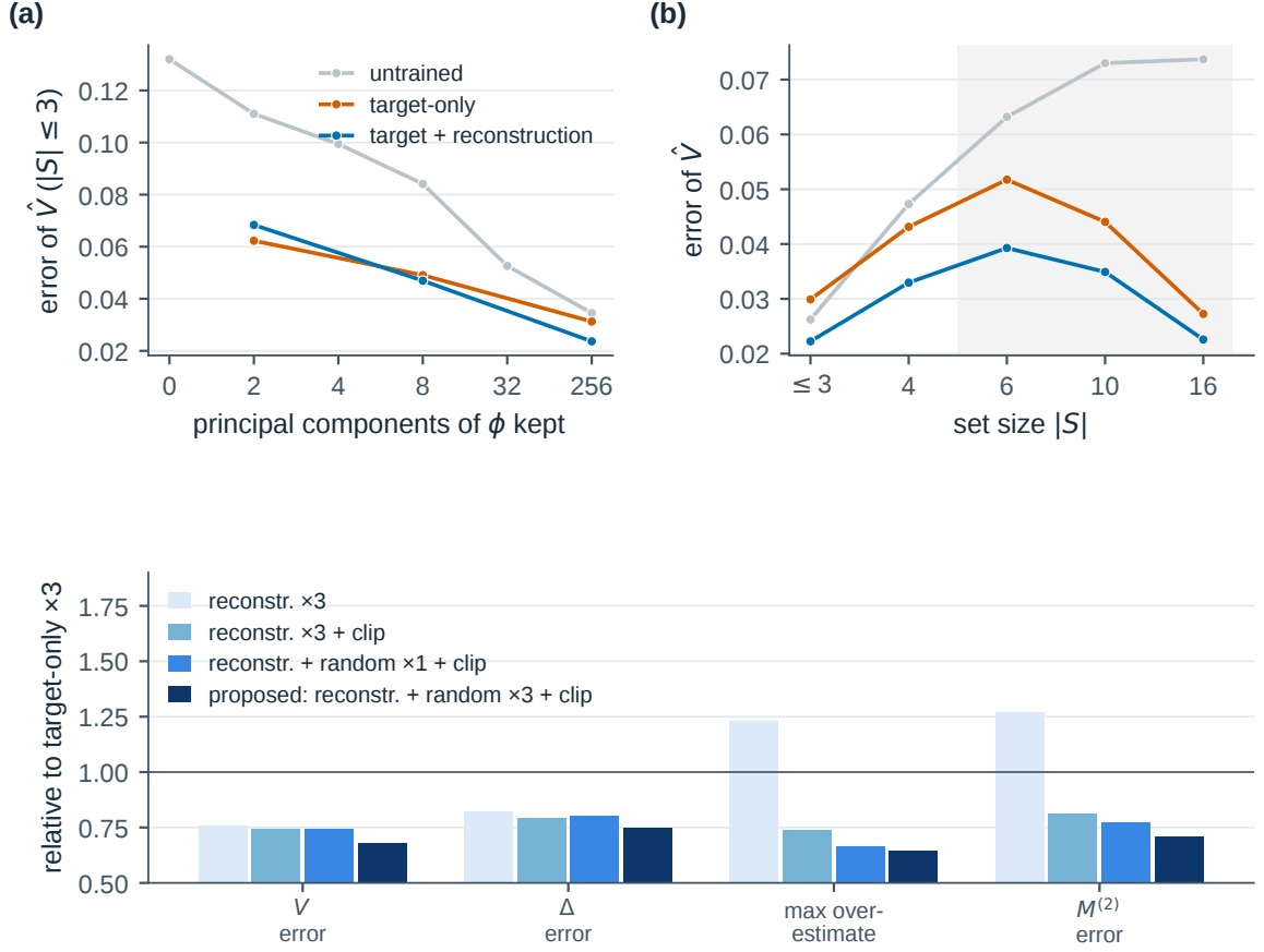
Figure 13: Representation and stability diagnostics. (a) Set-value error when only leading principal components are retained. (b) Error with increasing set size; shaded queries use a gradient-boosting reference. (c) Effects of clipping and the random feature branch on set-value, marginal and maximum-risk errors, relative to the target-only three-seed configuration.
