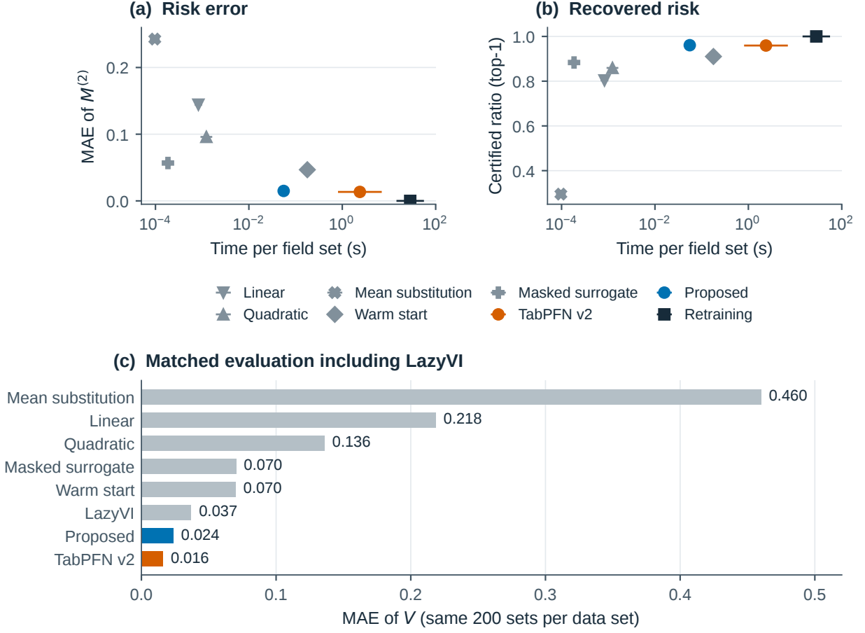
Figure 9: Comparison with other estimators over ten targets. (a) Error of M^{(2)} and (b) certified top-1 ratio against the time per field set (all targets of a data set; bars: range over data sets); retraining defines the ground truth. (c) Error of V on the same 200 sets per data set for every method, including LazyVI, which was too slow to run on all sets.
