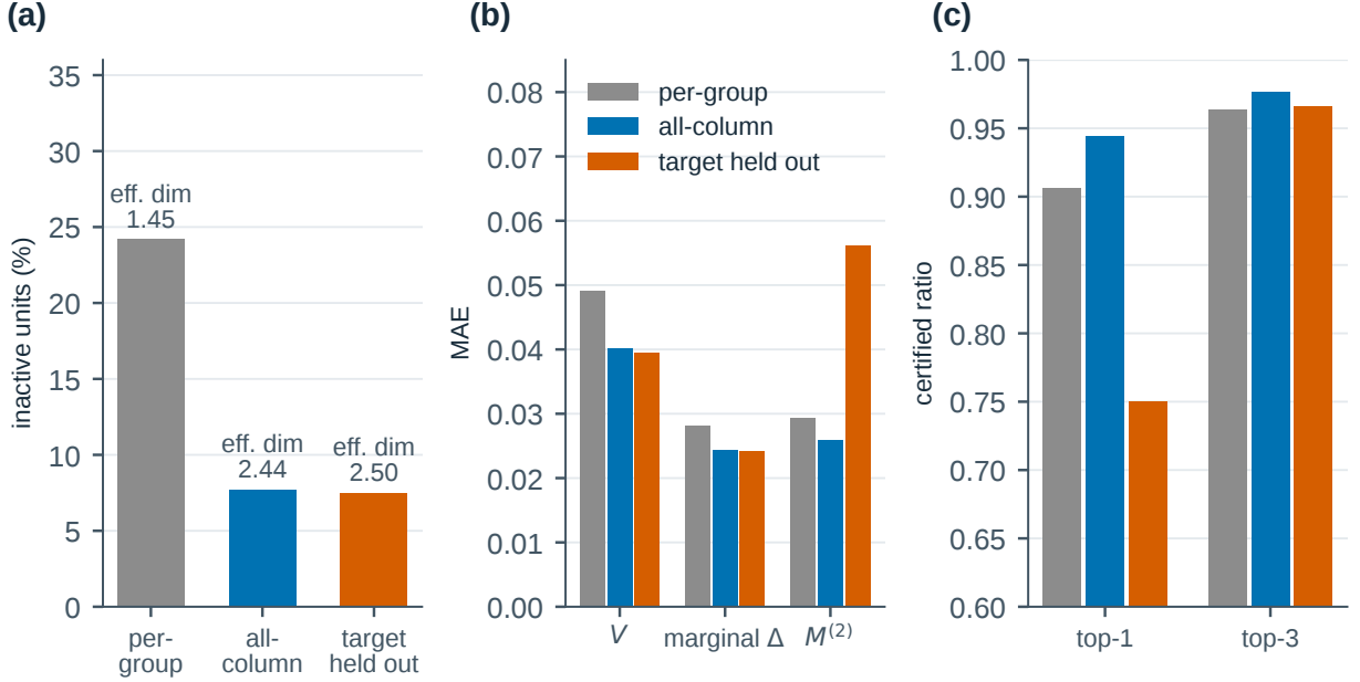
Figure 11: Backbone scope on the four PJM/CAISO targets (per-set readout on each backbone alone, three seeds): (a) inactive hidden units and effective dimension, (b) error of V , of marginals and of M^{(2)} , (c) certified ratios.
