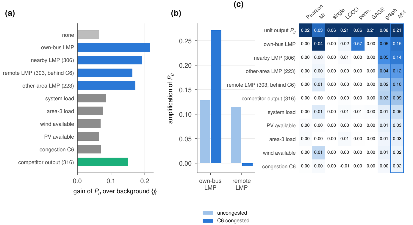
Fig. 3. Controlled mechanism: private offer markup of unit 313_CC_1 ( \pm 5\% ). (a) Gain of the unit output P_g over each single background. (b) Amplification of P_g by the own-bus and the remote price in uncongested hours and in hours when line C6 is congested. (c) Scores of eight methods for the eleven fields (colour normalized per column; last column M^{(2)} ).
