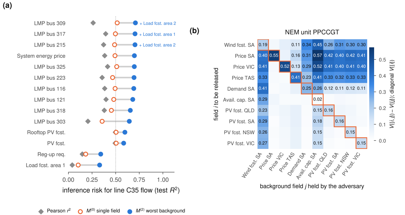
Fig. 5. (a) Field profile for the hourly flow on RTS line C35 (14 fields with the largest M^{(2)} ): Pearson r^2 , single-field risk and worst-background risk, with the witness background for the three riskiest fields. (b) Gain matrix for NEM unit PPCCGT: entry (i, j) is V(\{i, j\}) - V(\{j\}) , the diagonal is V(\{i\}) ; values below 0.10 are not printed.
