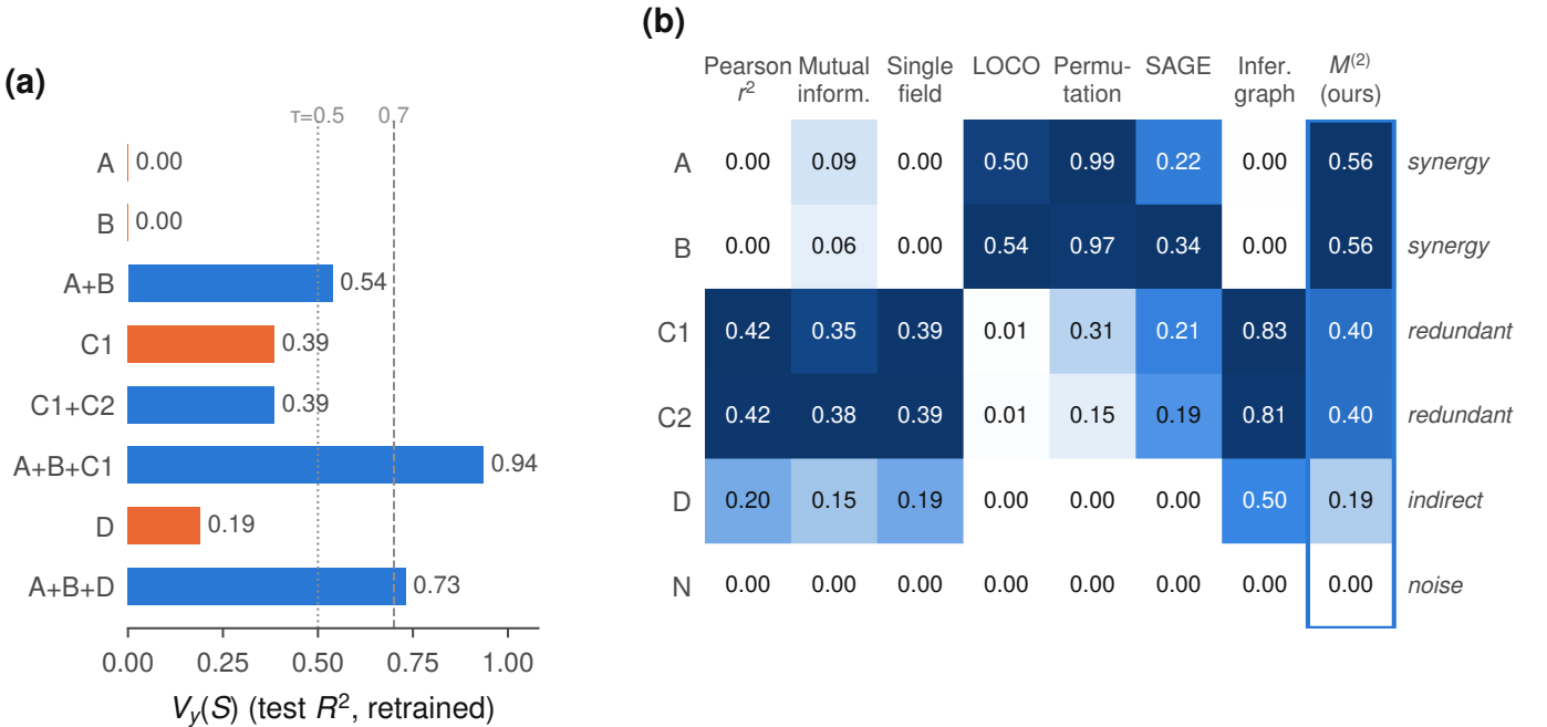
Fig. 12. Synthetic mechanism example. (a) Retrained inferability of selected sets. (b) Scores of eight methods (colour normalized per column); the last column is M^{(2)} .
