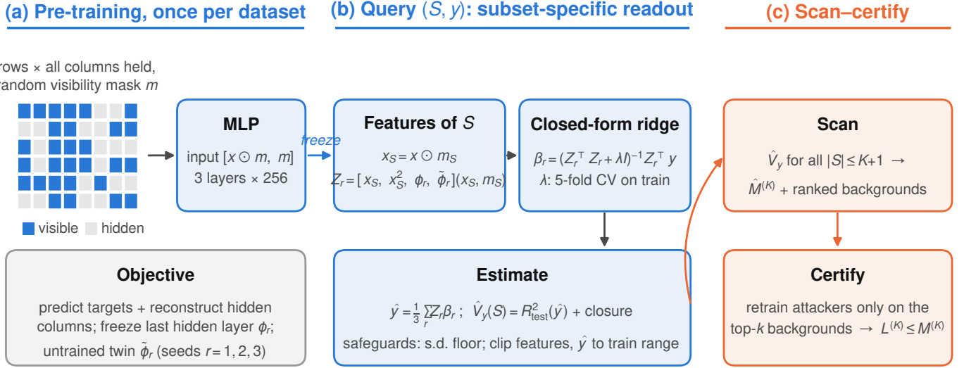
Fig. 2. The amortized attacker. (a) One backbone is pre-trained under random visibility masks on the auditor’s data, to predict the targets and reconstruct the hidden columns, and frozen. (b) A query (S, y) solves a ridge readout in closed form on the features of S —from the pre-trained backbone and an untrained network of the same architecture—per seed, and averages the predictions. (c) The Scan proposes backgrounds per field; retraining only these certifies a lower bound on M_{i \rightarrow y}^{(K)} .
