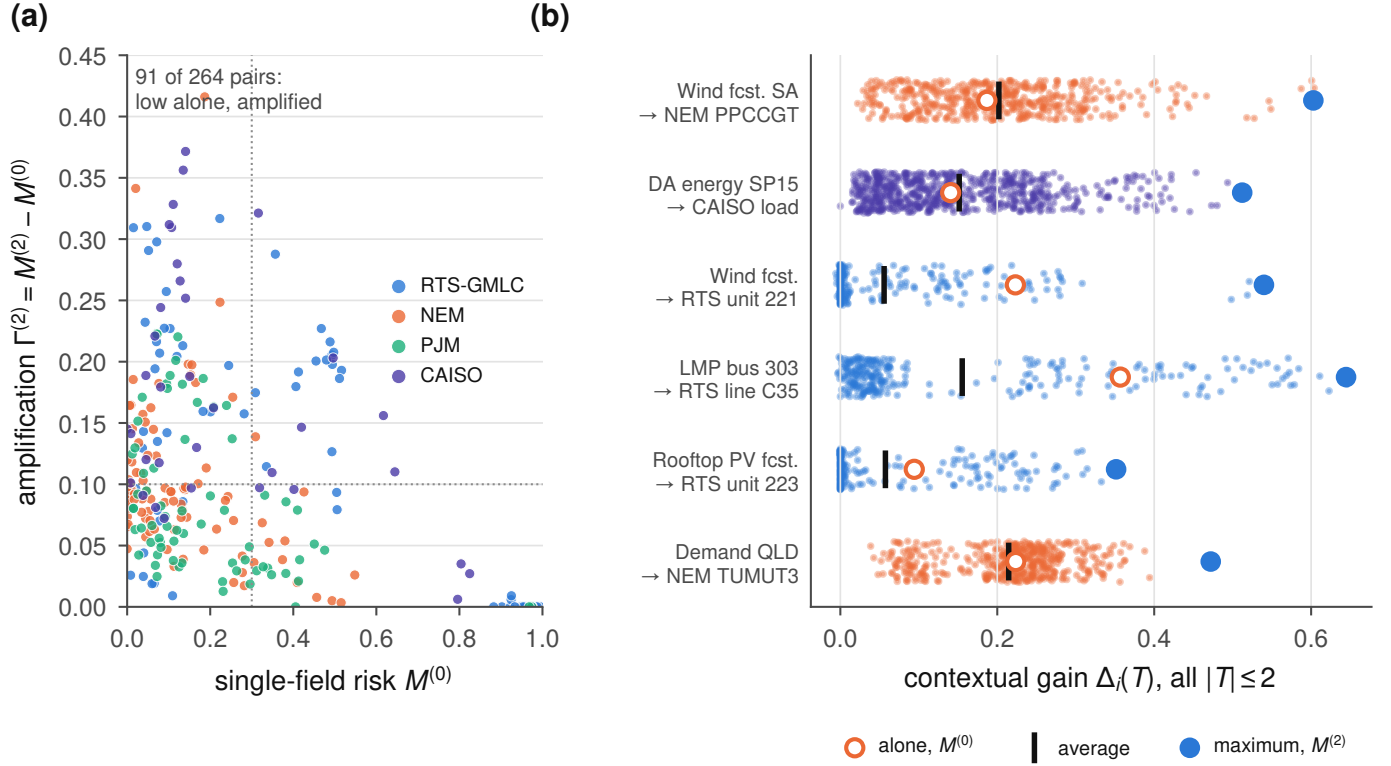
Fig. 6. Background amplification over ten targets. (a) Single-field risk versus amplification \Gamma^{(2)} for every field–target pair. (b) Contextual gains of the most amplified field of six targets over all backgrounds of at most two fields, with the single-field value, the average over backgrounds and the maximum.
