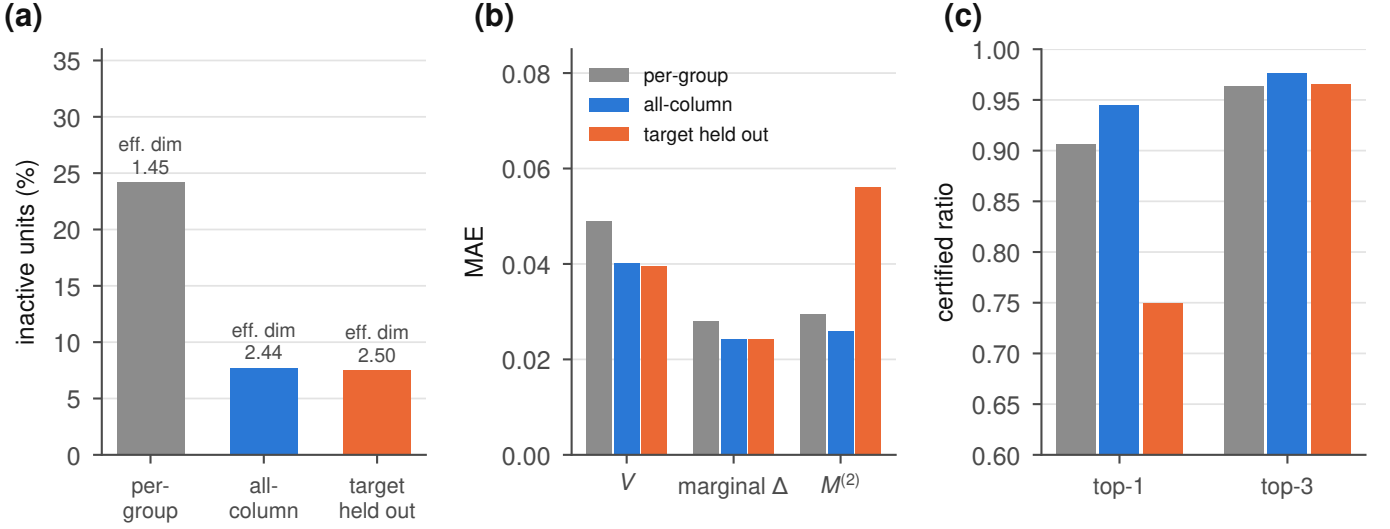
Fig. 11. Backbone scope on the four PJM/CAISO targets (per-set readout on each backbone alone, three seeds): (a) inactive hidden units and effective dimension, (b) error of V , of marginals and of M^{(2)} , (c) certified ratios.
