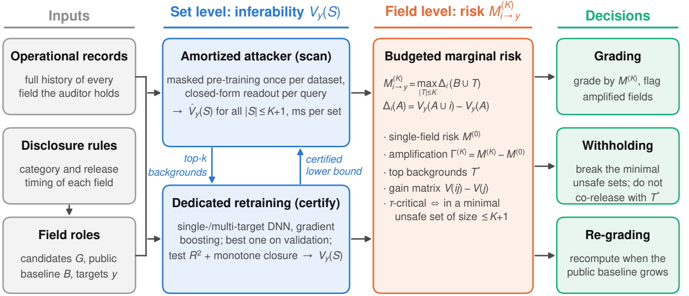
Fig. 1. Audit framework. Disclosure rules fix field roles. Set-level inferability V_y(S) is defined by dedicated retraining and scanned by an amortized attacker; the scan proposes, for every field, backgrounds that are certified by retraining. The field-level profile—single-field risk, background amplification and top backgrounds—supports grading, withholding and re-grading.
