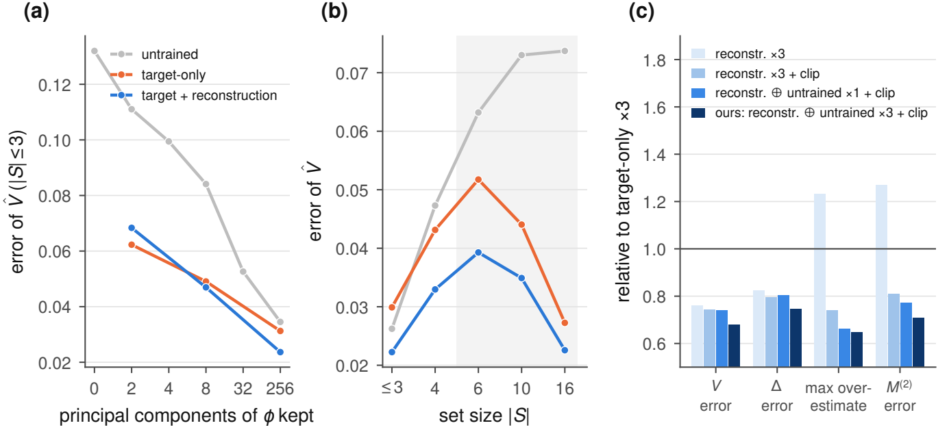
Fig. 8. Why target-only masked pre-training adds little, and the repair (ten targets). (a) Error of \hat{V} when the backbone features of each set are truncated to their r leading principal components (200 sets of size \leq 3 per data set, four data sets). (b) Error of \hat{V} against set size; shaded: gradient-boosting ground truth. (c) Errors of reconstruction pre-training relative to target-only pre-training (three seeds each), without and with clipping predictions to the training range, and with concatenated untrained features (one seed, mean over three; three seeds: ours): set values, marginals, the largest overestimate of a marginal per field, and M^{(2)} .
