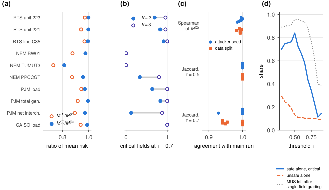
Fig. 10. Robustness. (a) Saturation of mean field risk in the background budget. (b) Share of \tau -critical fields at \tau = 0.7 with K = 2 (filled) and K = 3 (open). (c) Agreement of reruns with different attacker seeds or data splits with the main run. (d) Threshold sweep over ten targets: fields that are safe alone but critical (solid), fields unsafe alone (dashed), and minimal unsafe sets left after single-field grading (dotted).
