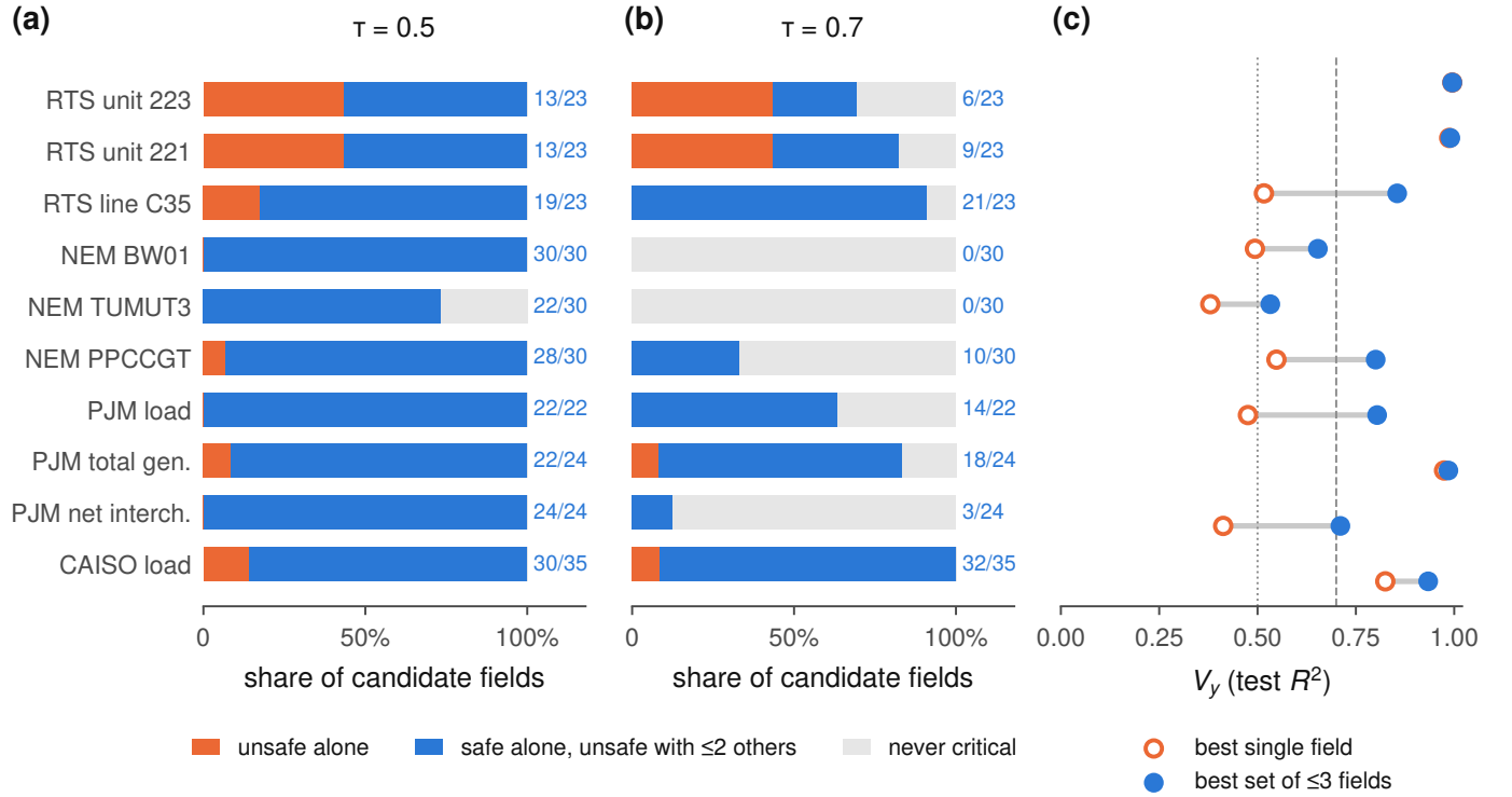
Fig. 4. Share of candidate fields that are unsafe alone (orange), safe alone but critical with at most two background fields (blue), or never critical (grey), at (a) \tau = 0.5 and (b) \tau = 0.7 ; numbers give combination-critical fields over all candidates. (c) Best single field versus best set of at most three fields.
