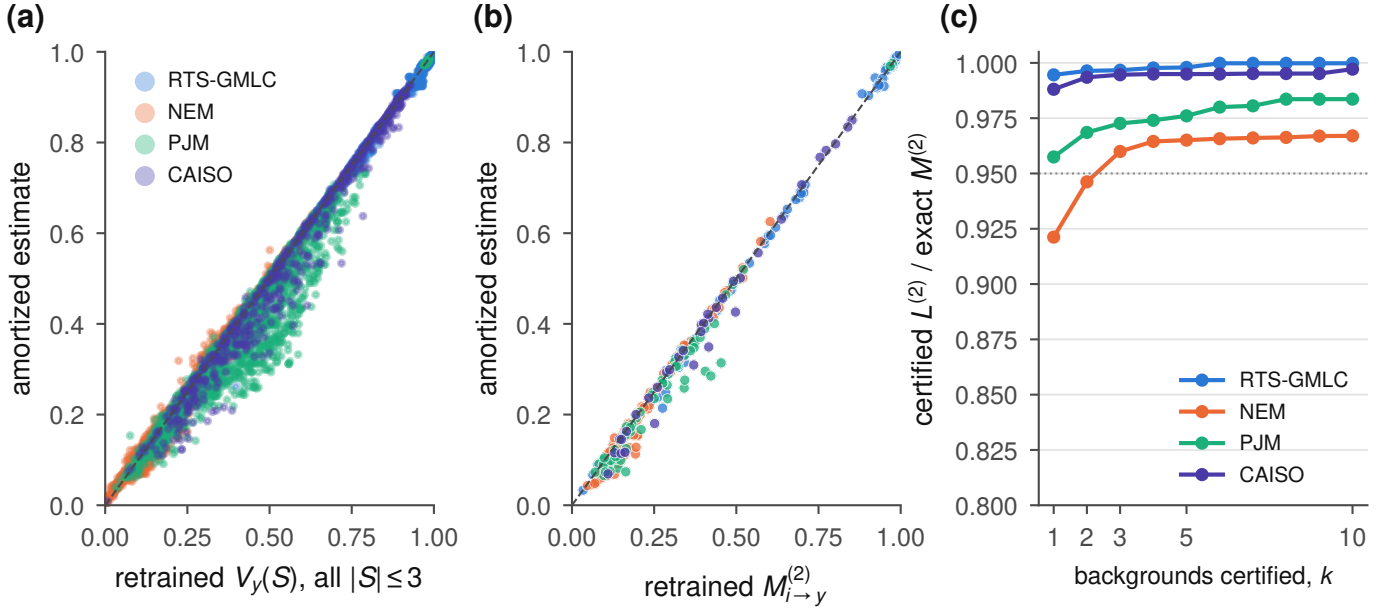
Fig. 7. Amortized estimates against retrained ground truth. (a) \hat{V}_y(S) for sets of size \leq 3 (random subsample). (b) \hat{M}^{(2)} for every field and target. (c) Certified lower bound over exact M^{(2)} when the top- k scanned backgrounds per field are retrained.
