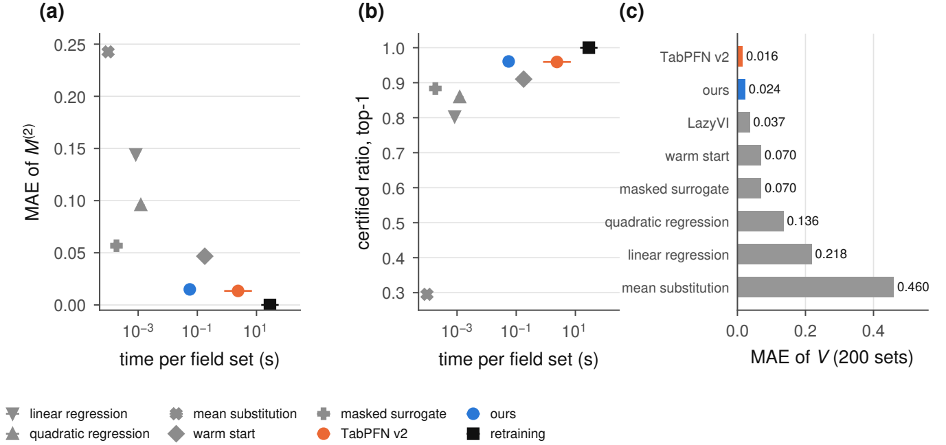
Fig. 9. Comparison with other estimators over ten targets. (a) Error of M^{(2)} and (b) certified top-1 ratio against the time per field set (all targets of a data set; bars: range over data sets); retraining defines the ground truth. (c) Error of V on the same 200 sets per data set for every method, including LazyVI, which was too slow to run on all sets.
