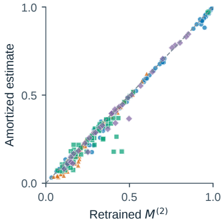
(b) Field risk
