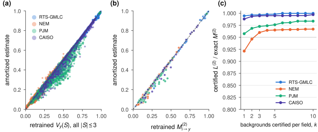
Figure 7: Amortized estimates against retrained ground truth. (a) \hat{V}_y(S) for sets of size \leq 3 (random subsample). (b) \hat{M}^{(2)} for every field and target. (c) Certified lower bound over exact M^{(2)} when the top- k scanned backgrounds per field are retrained.
