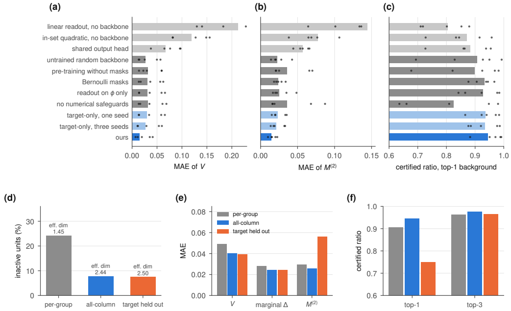
Figure 8: (a–c) Estimator comparison and ablation over ten targets (bars: mean; dots: data sets); light grey: no per-set readout or no backbone; dark grey: one-seed ablations of a target-only backbone; light blue: target-only pre-training; blue: ours. (d–f) Backbone scope on the four PJM/CAISO targets: inactive hidden units and effective dimension, error of V , of marginals and of M^{(2)} , and certified ratios.
