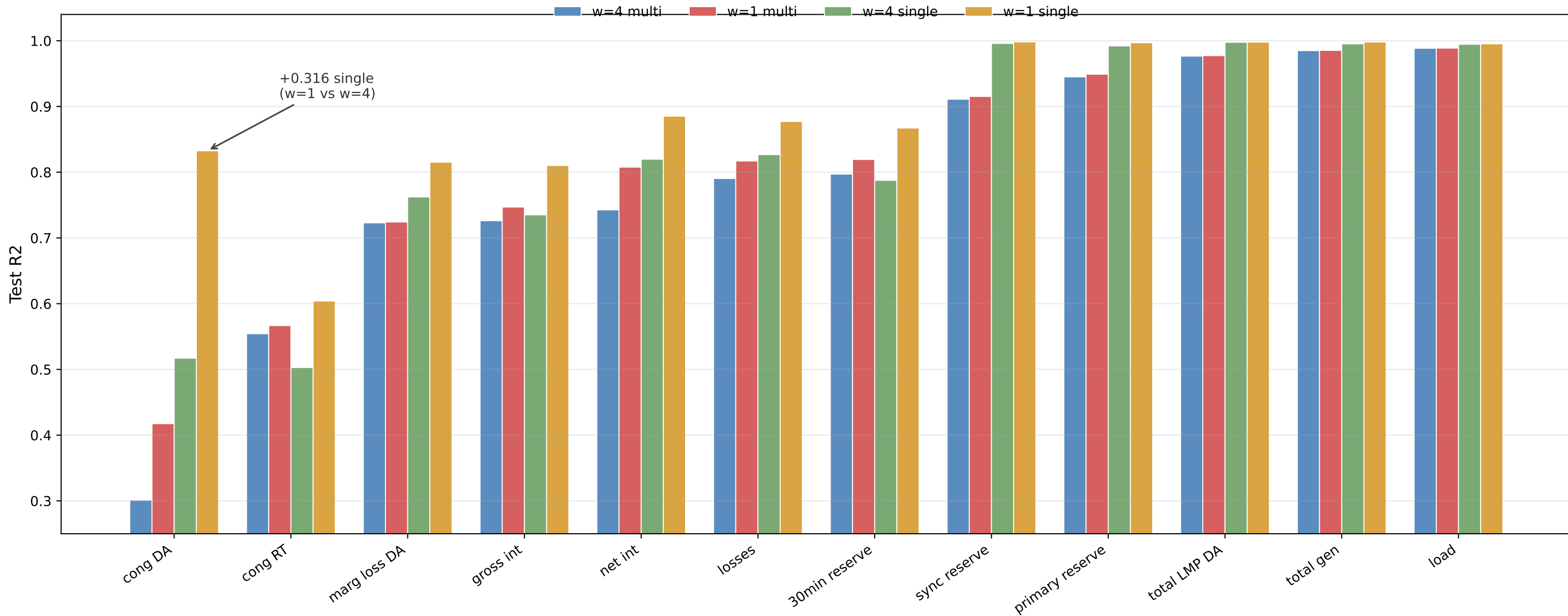
DNN32 Window Ablation: Multi vs Single R2
