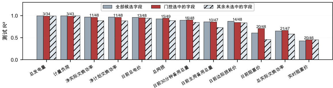
图 3 全部字段、选中字段与未选中字段的还原精度对比 Fig. 3 Recovery accuracy of all, selected and unselected fields
