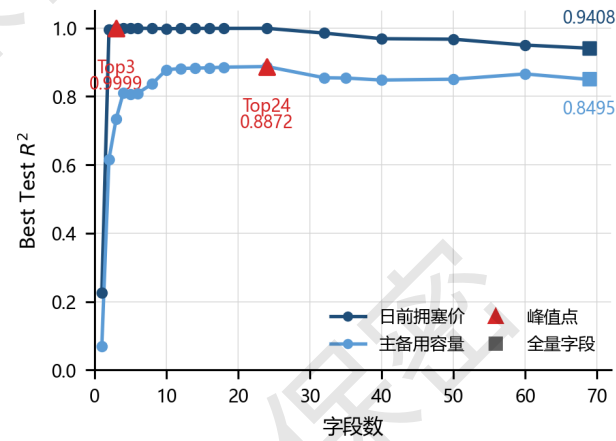
图 12 按 L1 门控排名逐步增加字段数的测试 R^2 变化 Fig. 12 Test R^2 variation with incrementally added Top-n features ranked by L1 gate values
