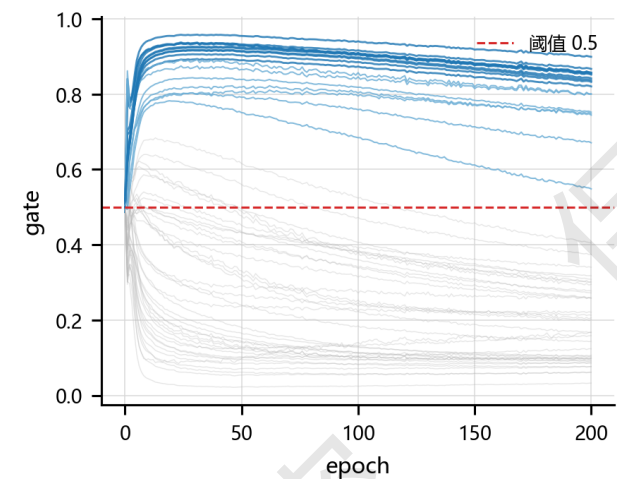
图 7 改进 L1 门控模型的门控值演化 Fig. 7 Gate value evolution of the improved L1-gated model
