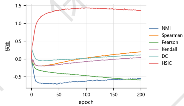
图 8 改进门控中指标权重的训练演化 Fig. 8 Evolution of metric weights in the improved gate
