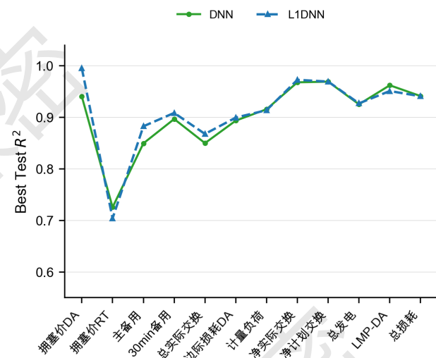
图 9 12 个目标字段上全量 DNN 与 L1 门控模型的测试 R^2 对比 Fig. 9 Comparison of test R^2 between all-feature DNN and L1-gated model across 12 targets
