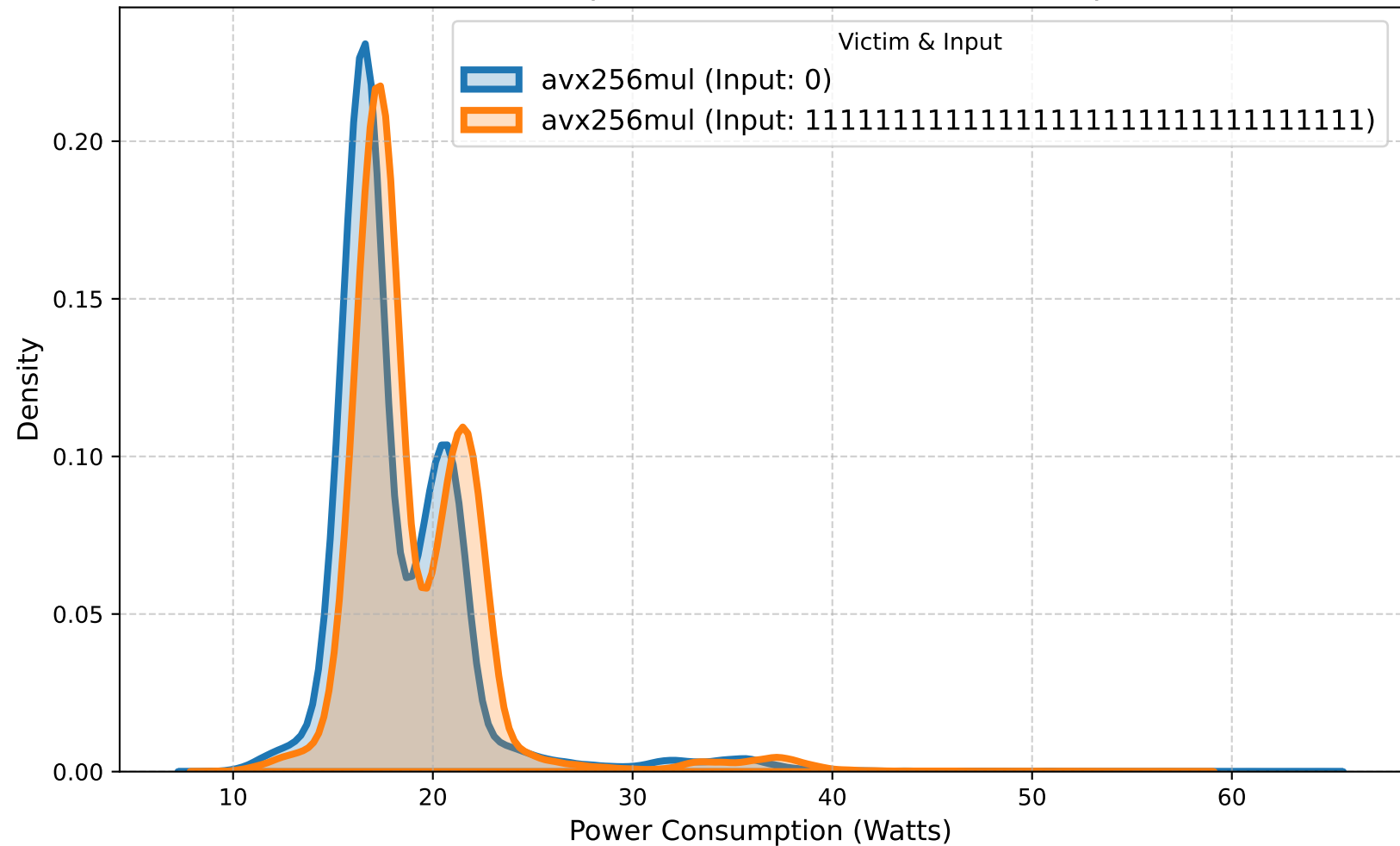
Power Consumption Distribution (300000 samples)
