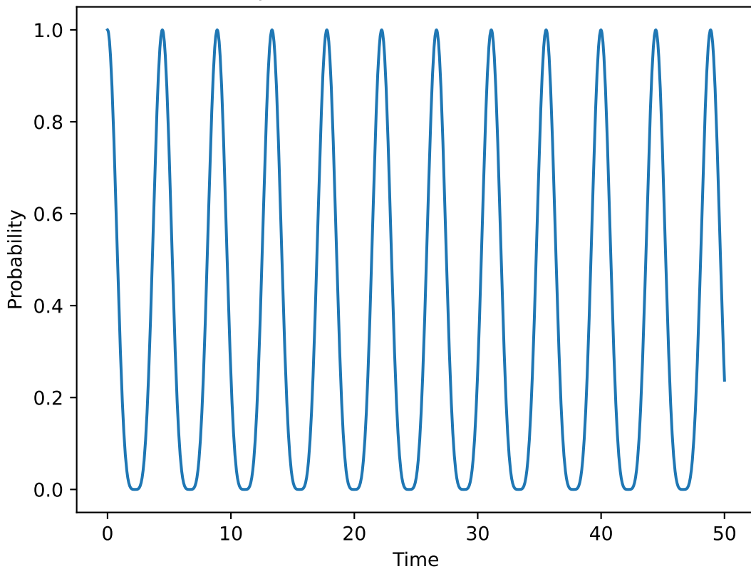
Overlap of Z2 State with Itself Over Time
