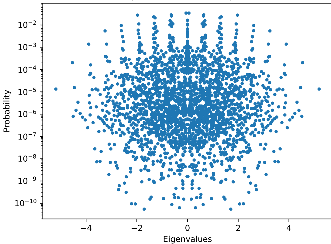
Overlap of Z2 State and Eigenstates
