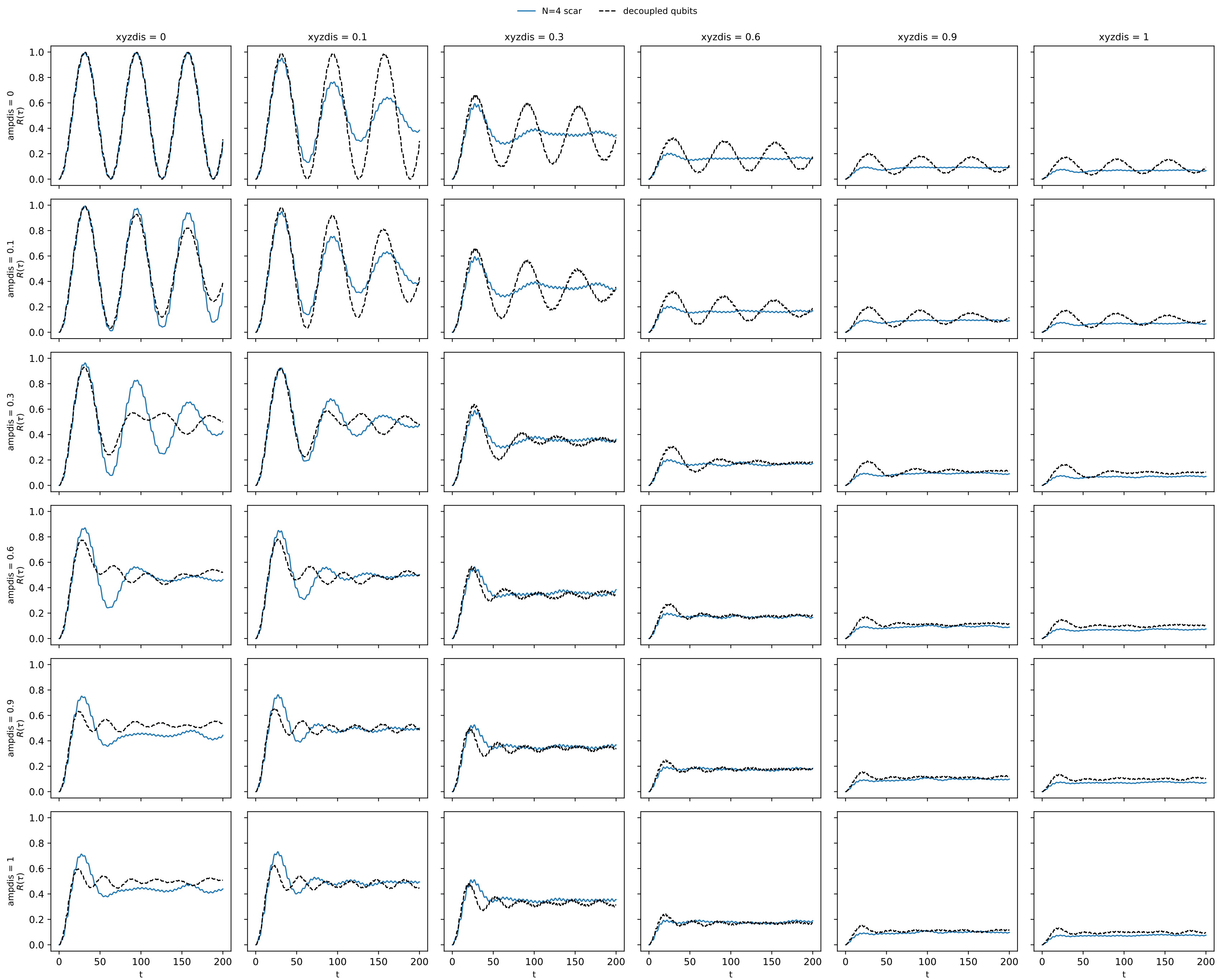
z-disorder (qubit reference: N=4)
