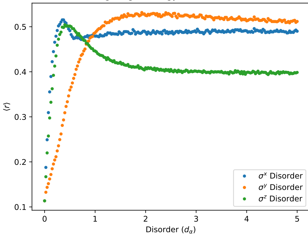
Average Eigenenergy Ratio vs. Disorder
