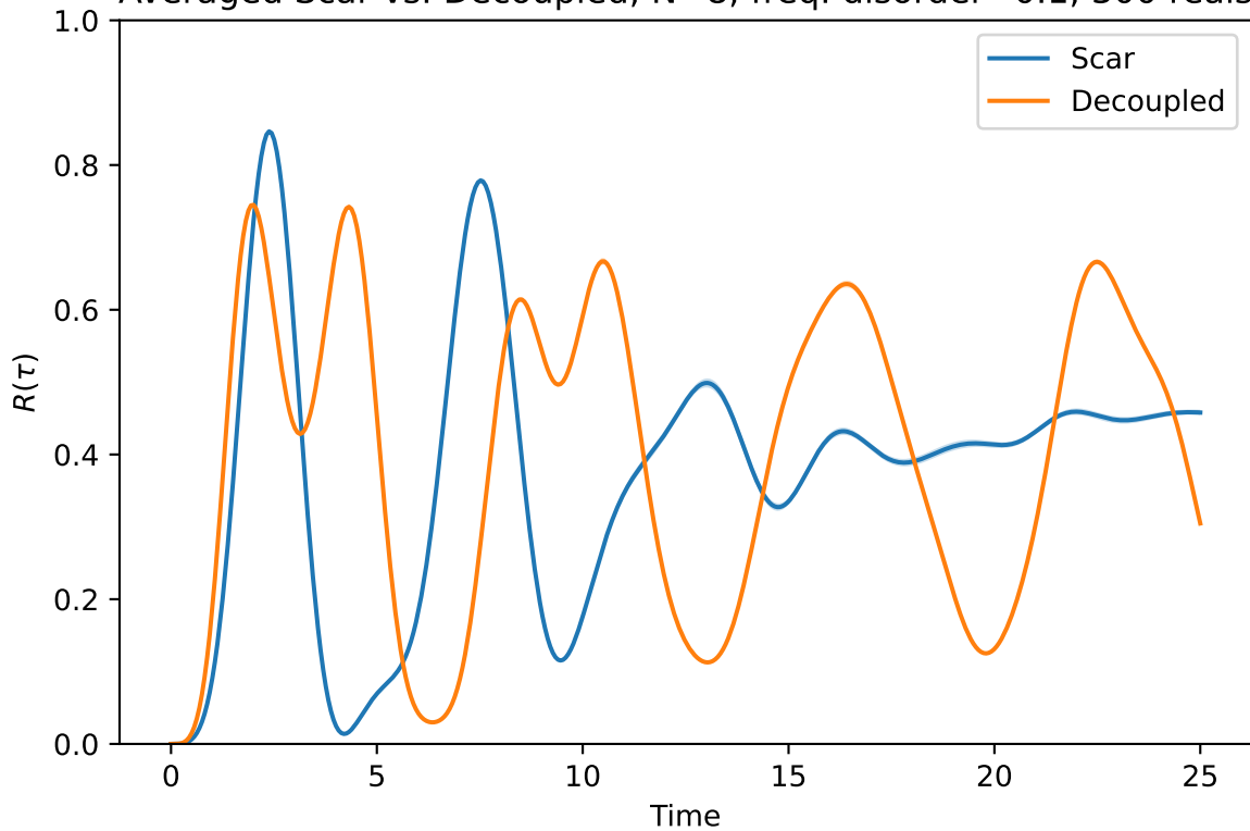
Averaged Scar vs. Decoupled, N=8 , freq. disorder=0.1, 300 reals
