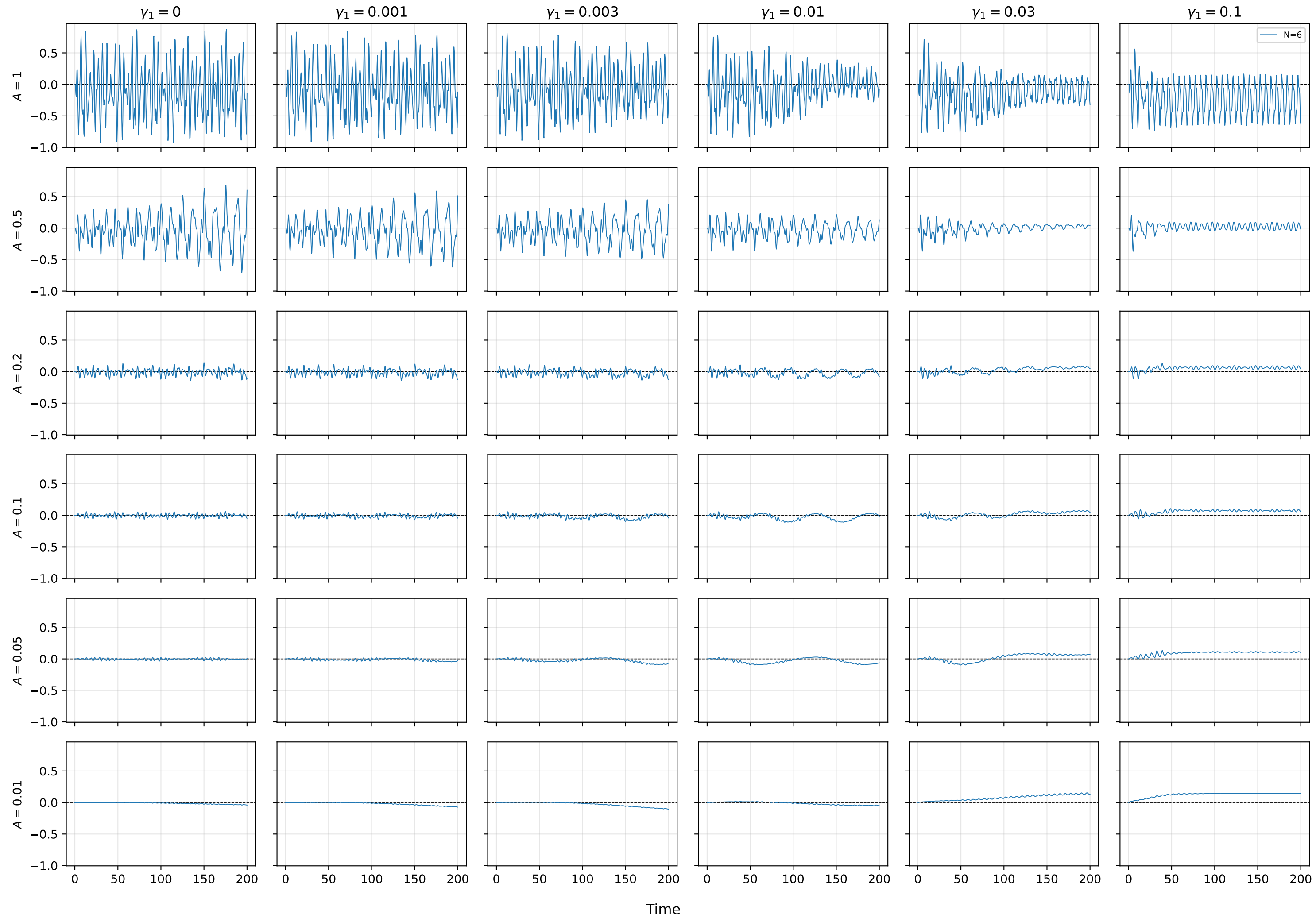
\mathcal{E}_{\text{scar}} - \mathcal{E}_{\text{qubit}} (per bandwidth), relaxation
