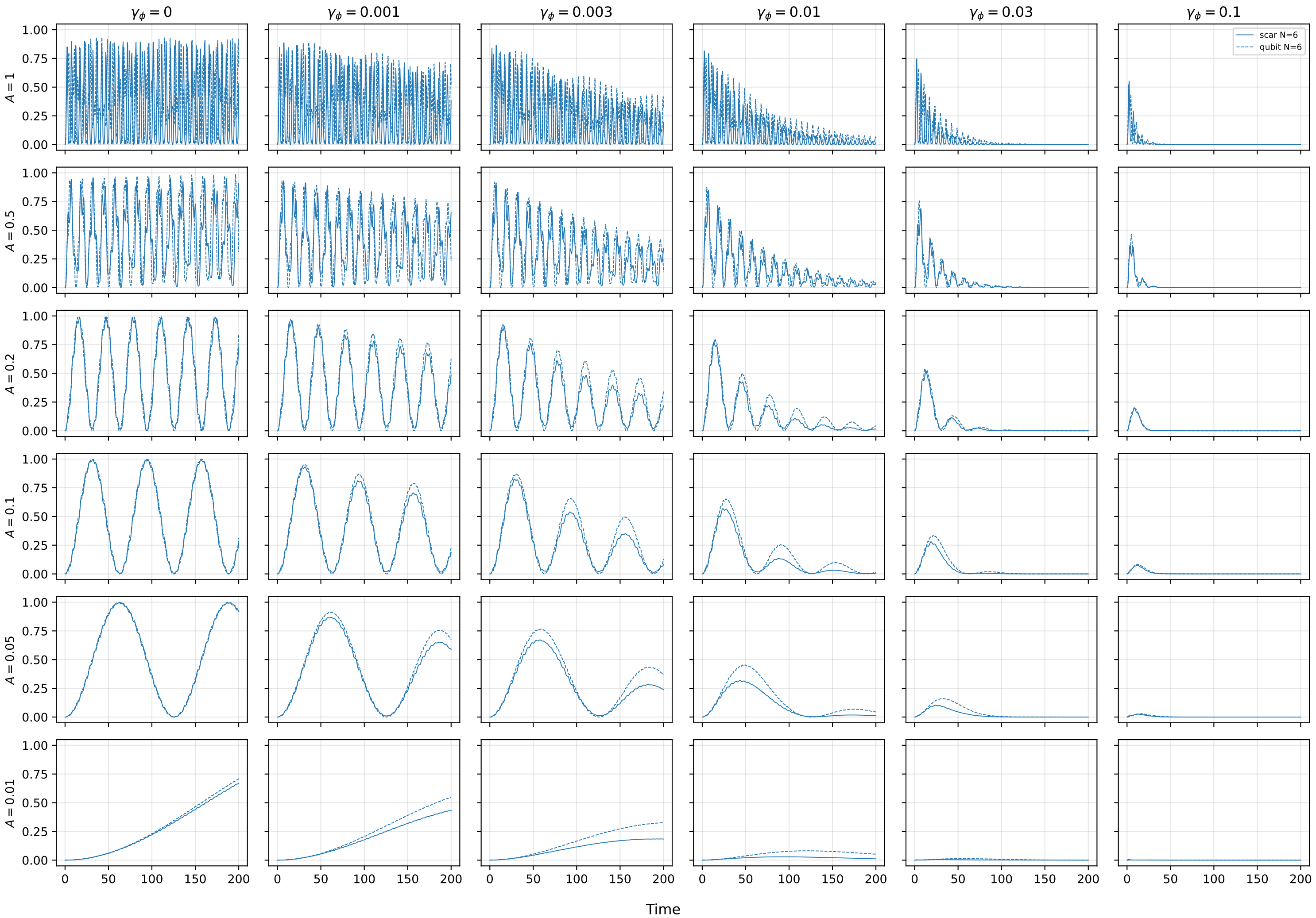
\mathcal{E}_{\text{scar}} (solid), \mathcal{E}_{\text{qubit}} (dashed), N = 6 , dephasing
