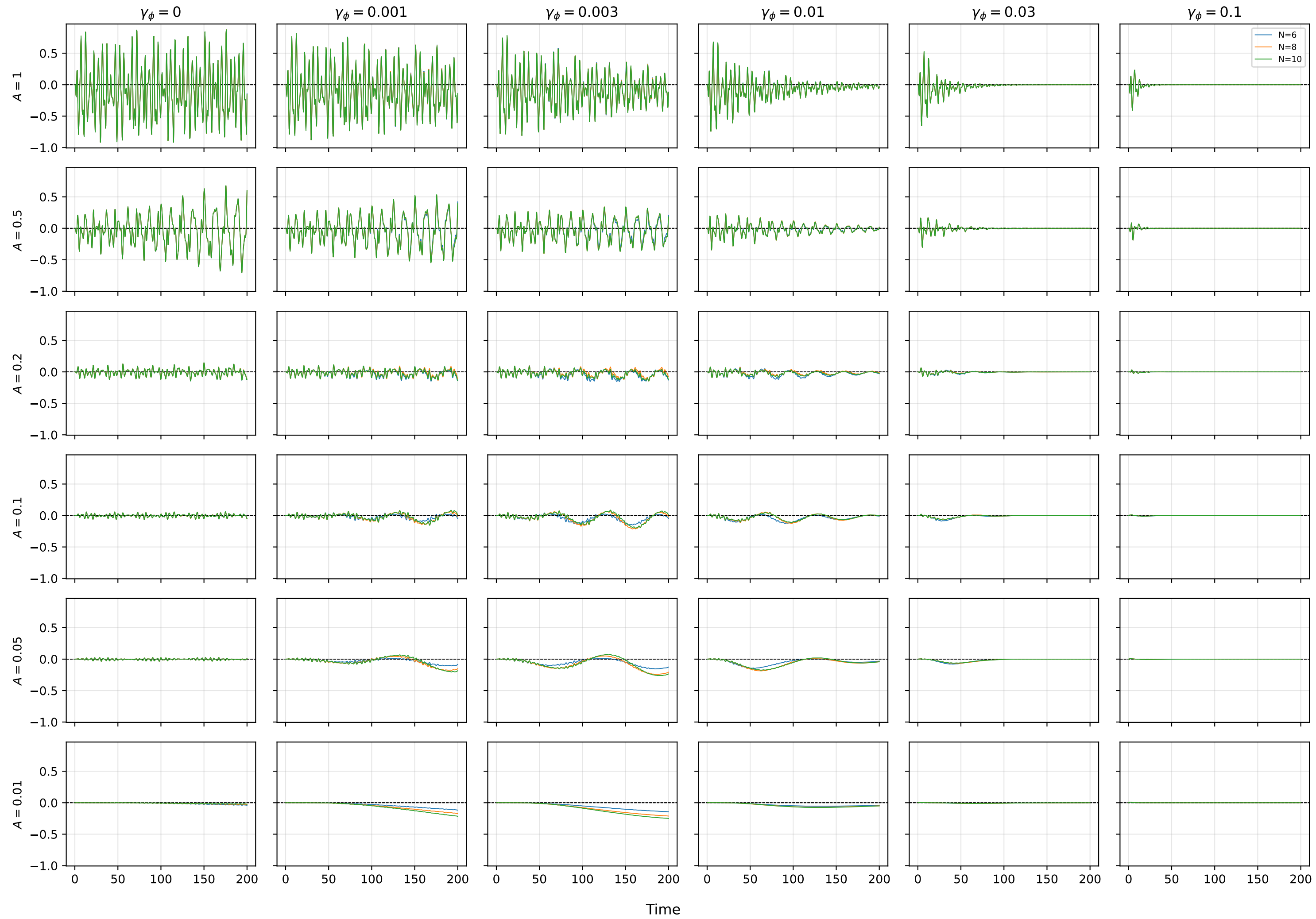
\mathcal{E}_{\text{scar}} - \mathcal{E}_{\text{qubit}} (per bandwidth), dephasing
