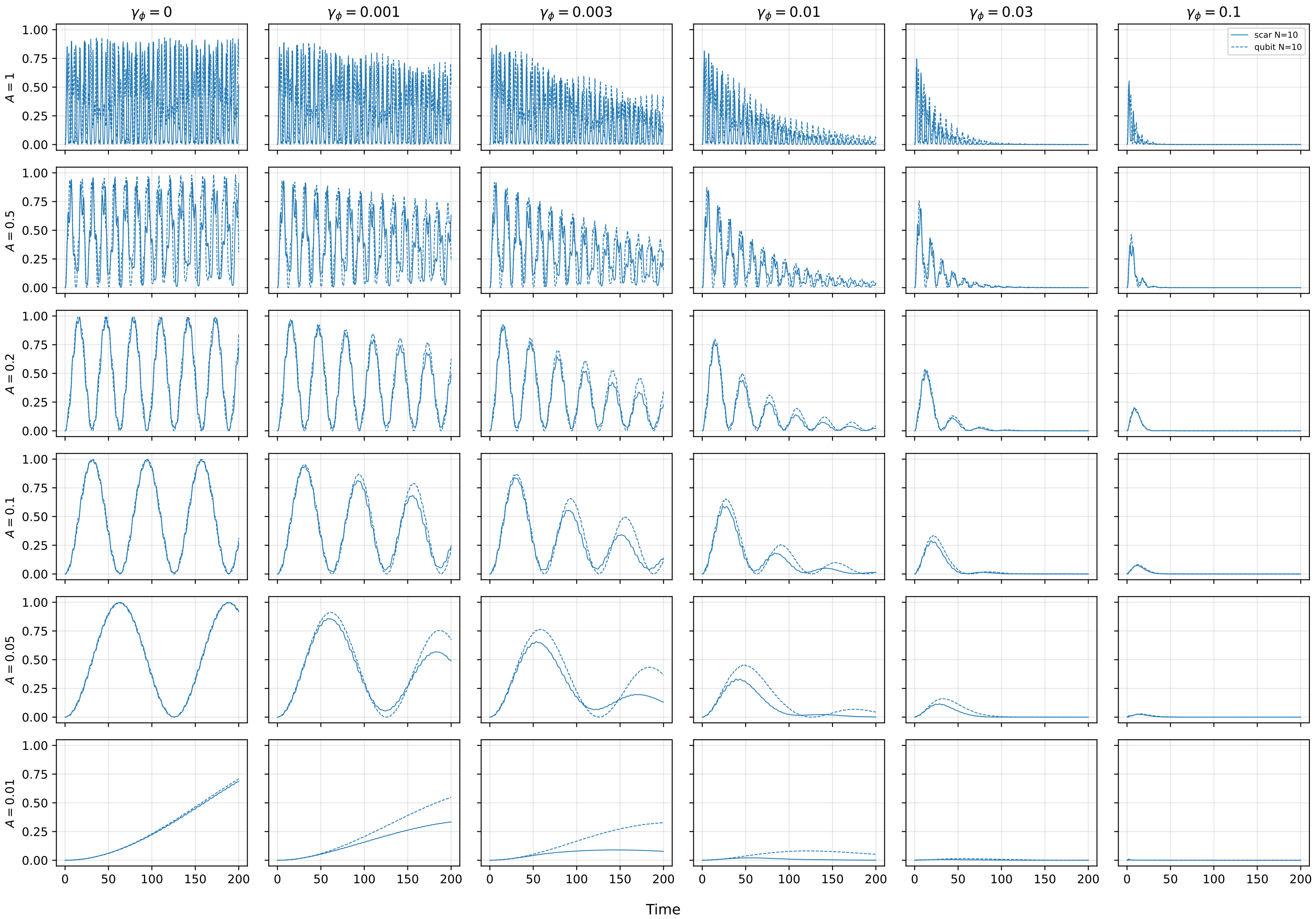
\mathcal{E}_{\text{scar}} (solid), \mathcal{E}_{\text{qubit}} (dashed), N = 10 , dephasing
