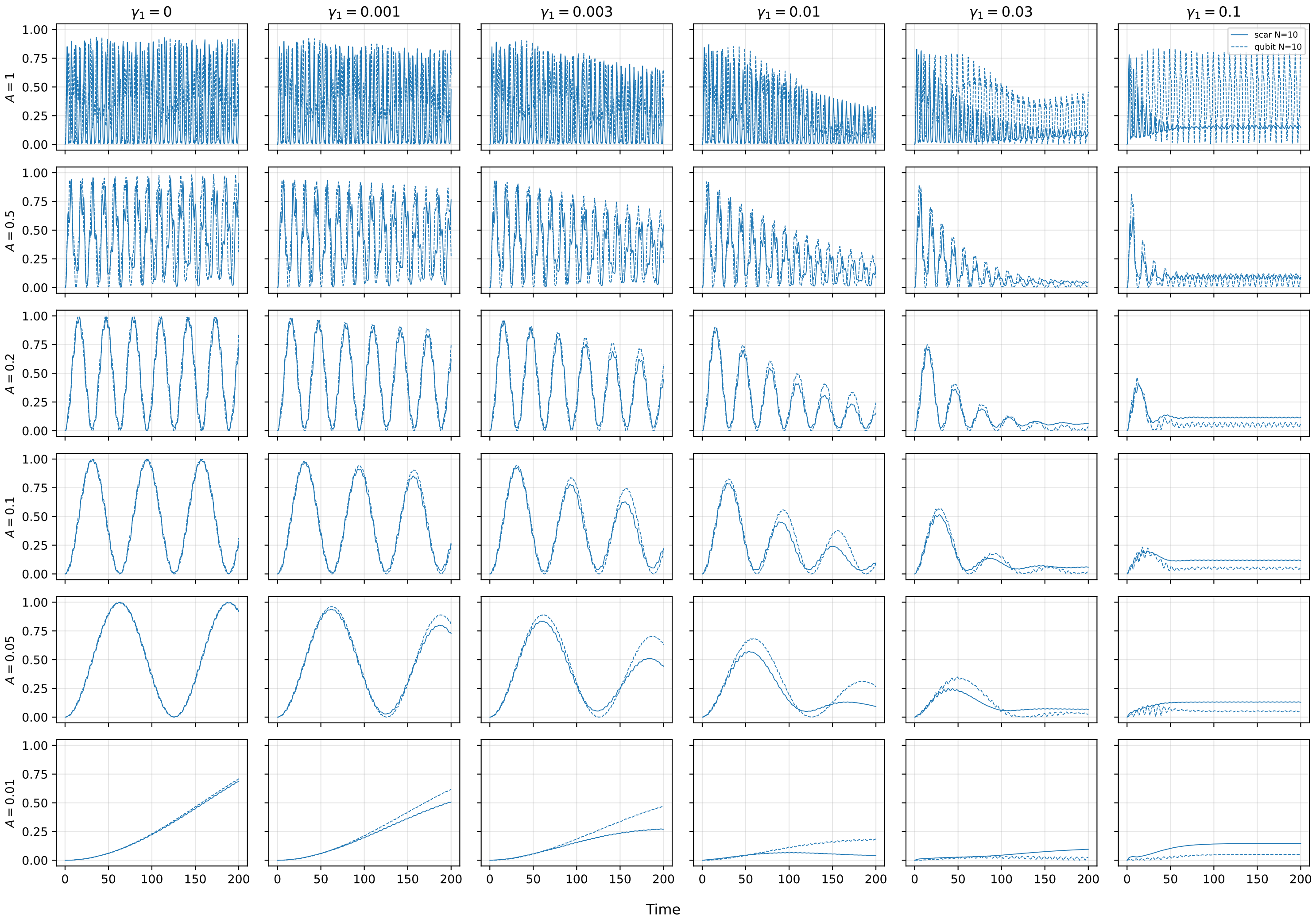
\mathcal{E}_{\text{scar}} (solid), \mathcal{E}_{\text{qubit}} (dashed), N = 10 , relaxation
