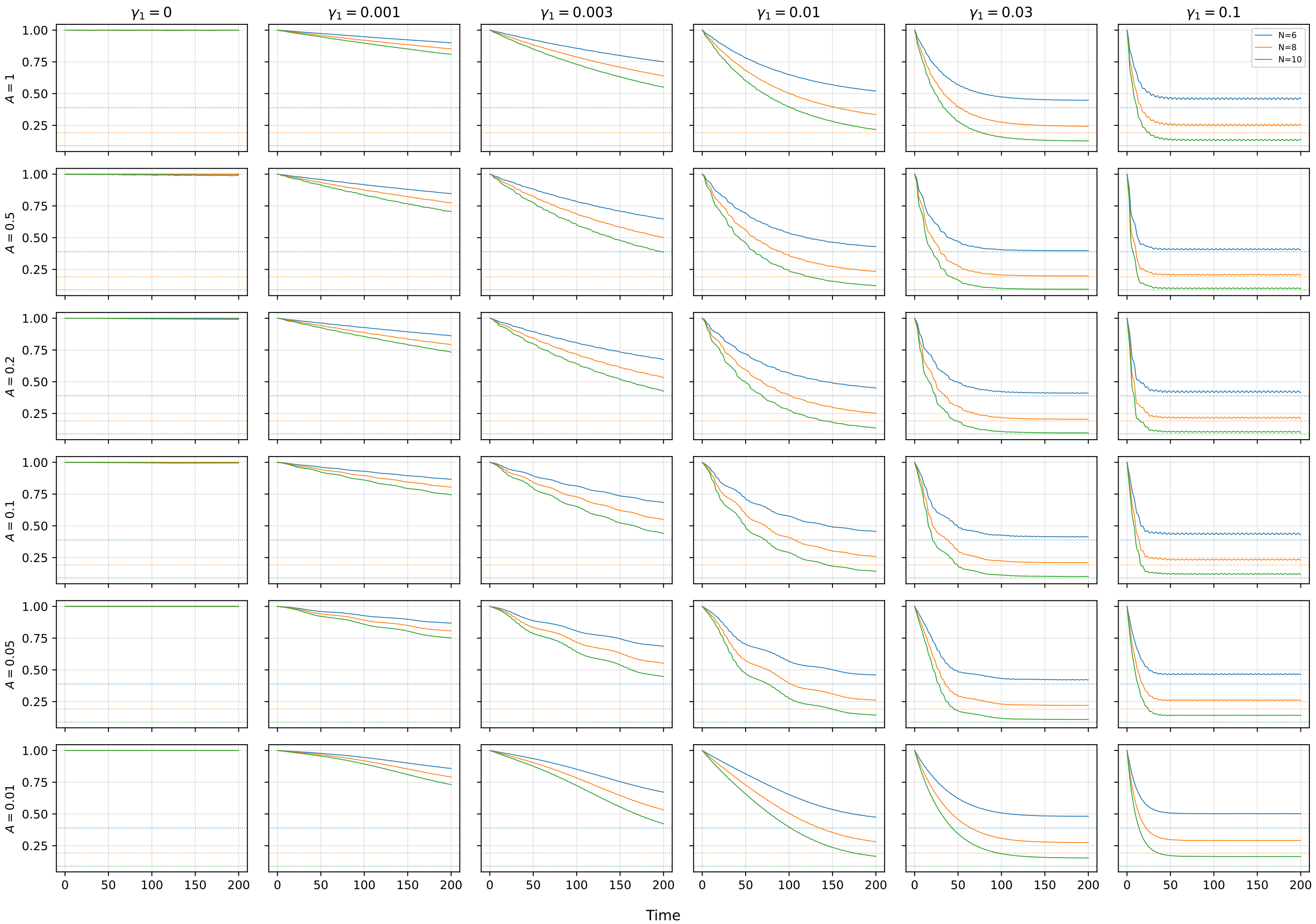
scar-tower population (dotted: maximally mixed value), relaxation
