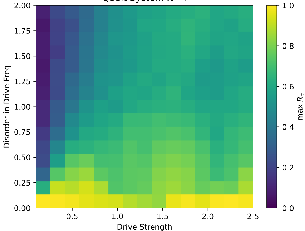
Qubit System N=4
