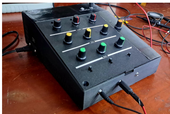
Figure 21: Final product
