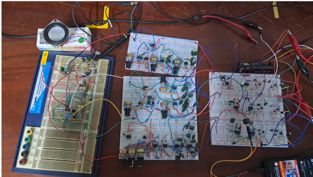
Figure 29: Breadboard testing.
