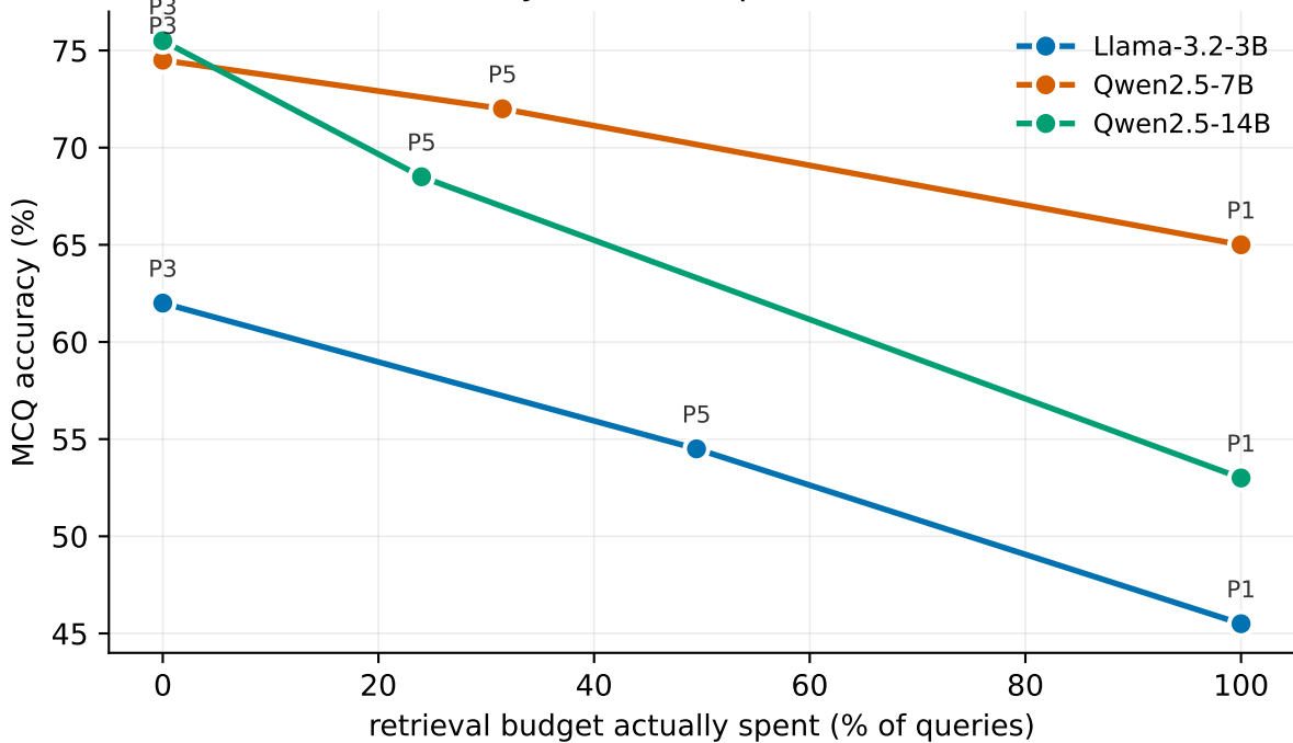
Retrieval costs accuracy on this corpus — at all three model scales
