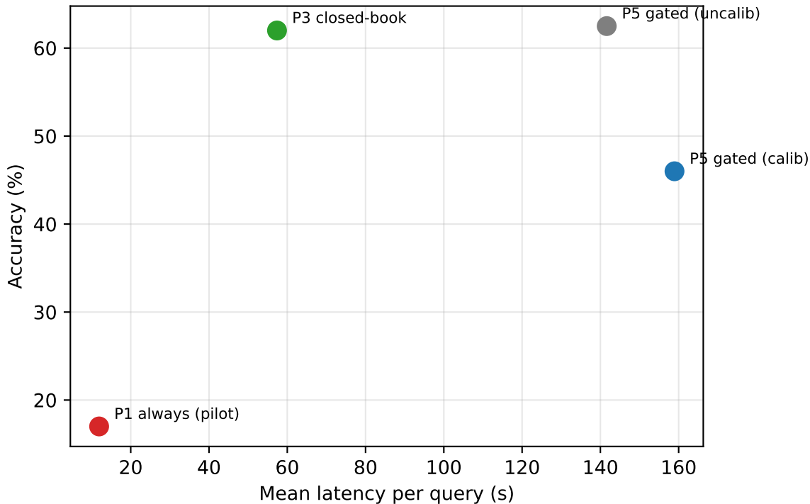
Accuracy vs latency on 200 MIRAGE MCQs (pilot corpus)
