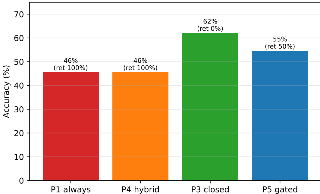
MCQ accuracy by policy on the real corpus (MedCorp)
