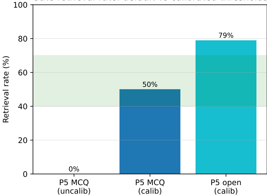
Gate retrieval rate: default vs calibrated thresholds
