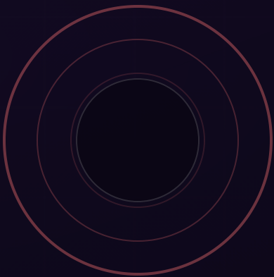
Single-asset speculation
