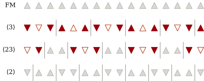
(b) structures at \kappa = 1/2 and the local field h of each spin position along y \rightarrow
