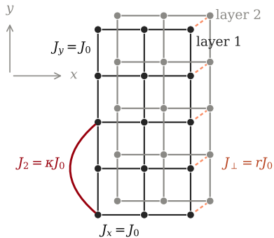
(a) bilayer, frustrated along y
