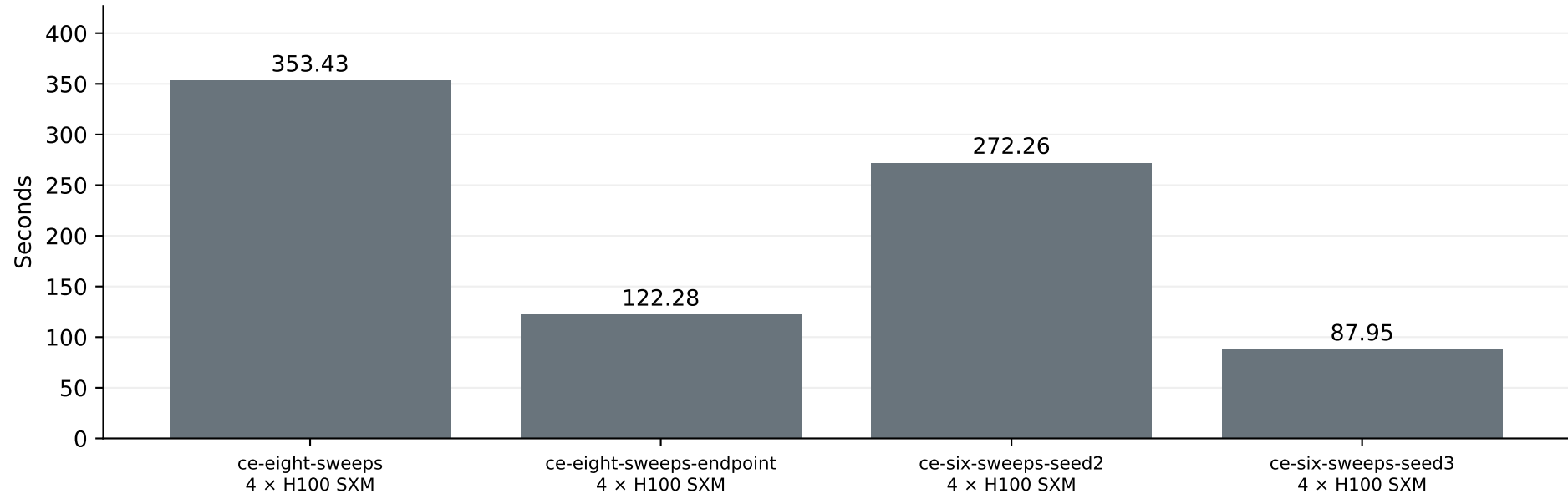
Observed sample call, including first-use compilation
