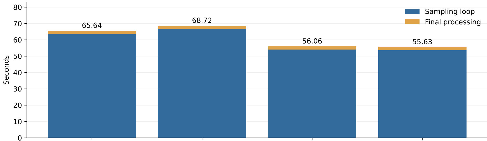
Sampling time with measured compilation excluded
