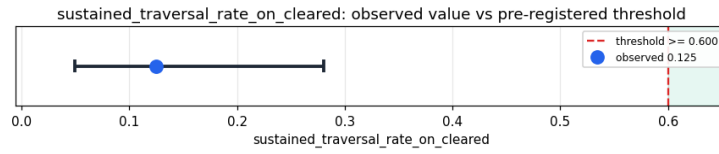
Figure 1: sustained_traversal_rate_on_cleared – observed value with Wilson 95% CI.
