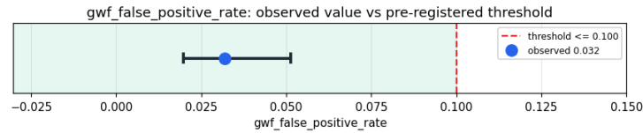
Figure 1: gwf_false_positive_rate – observed value with Wilson 95% CI.
