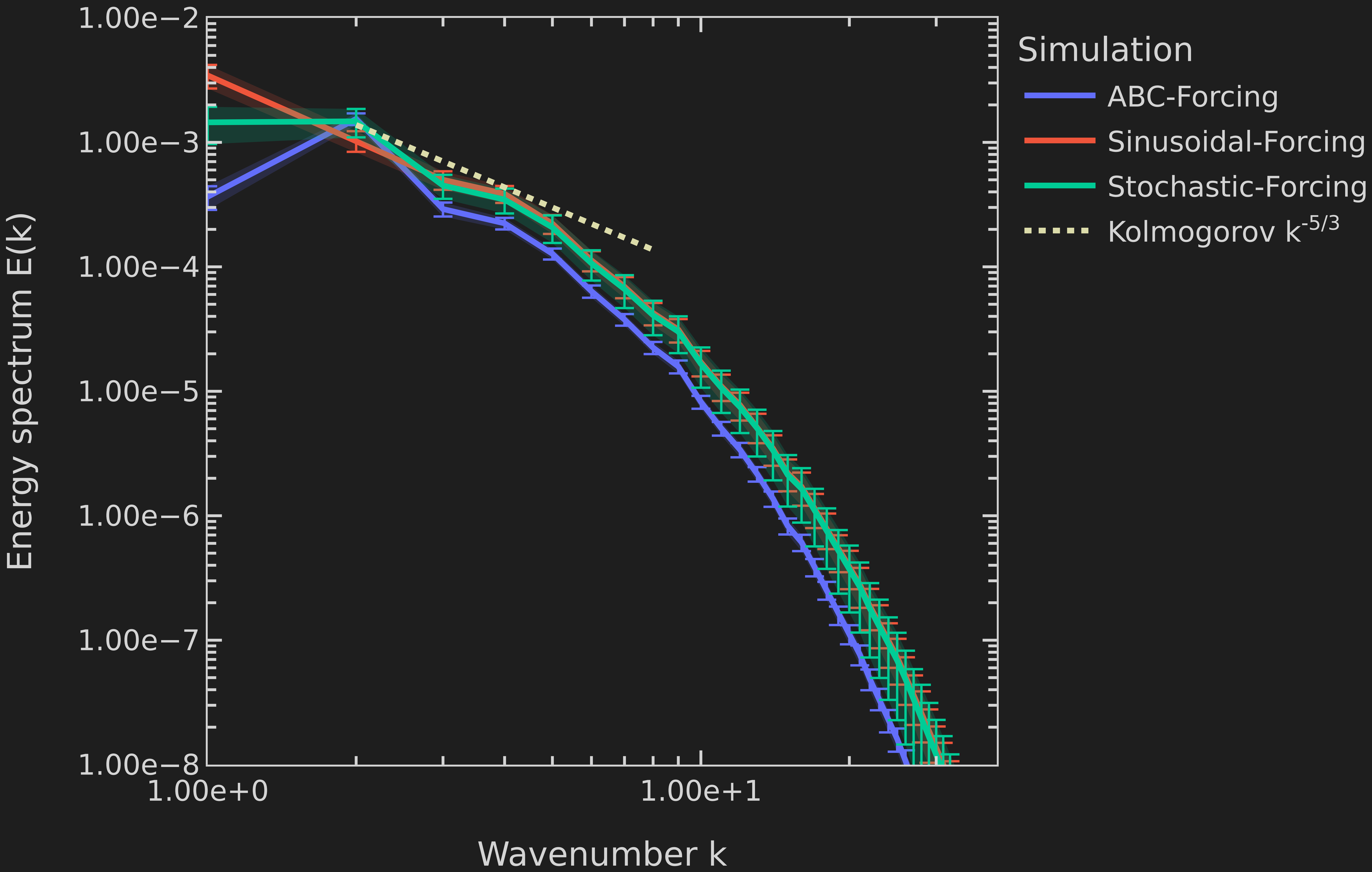
Energy spectra with same parameters & different forcing
