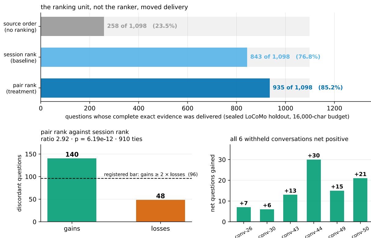
Figure 1. The sealed holdout. Six LoCoMo conversations withheld until the bars were locked, and the ranking unit is the whole difference. Complete exact-evidence delivery over 1,098 records at a 16,000-character budget: source order 258, session-score inheritance 843, own-cosine pair ranking 935. The gain/loss panel shows 140 against 48 with 910 ties, against the registered bar of gains at least twice losses — ratio 2.92, one-sided exact binomial p = 6.19e-12 . Every one of the six withheld conversations is net positive: +7, +6, +13, +30, +15, +21. Median packed characters differ by 2, so the treatment is not spending more. The result is bounded to availability and authorizes no reader claim. Sources: g6_holdout_outcomes.json 7be2668d21163c93, g7_result_integrity.json 890b4831d530e9a7, NF_004_PRE_REGISTRATION.md de2d5e05646b769c.
