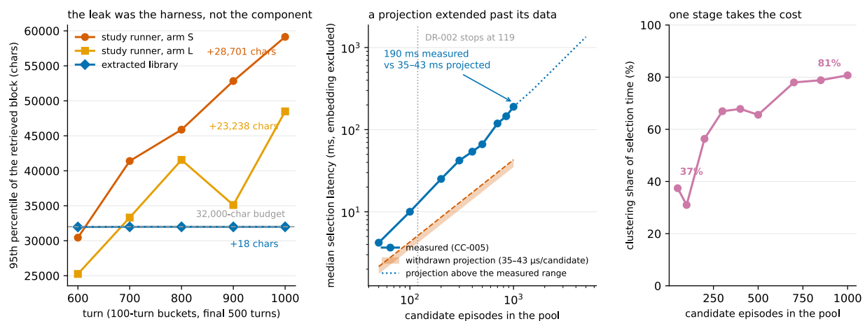
Figure 7. Growth and cost. The growth belonged to the harness; the cost was five times its projection. Left: the 95th percentile of the retrieved block per 100-turn bucket over the final 500 turns of the 1,000-turn run. In the study runner the block rises 23,238 characters in one arm and 28,701 in the other, still setting records in the last bucket; replayed through the extracted library at the same budget it moves +18 characters and breaches the budget on 0 of 1,000 turns — while truncating on 895 of them, so it is bounded because enforced, not because demand is small. Right: measured median selection latency against candidate count, with the withdrawn projection drawn as the range it actually published rather than a single point. 190 ms measured at 1,000 candidates, exponent 1.25 over 50–1,000, and clustering’s share rising from 37% to 81%. Values above 1,000 candidates are projections, drawn dashed. Sources: dx002_results.json f8ab79ab041cb3e3, ge0_growth_gate.json 350fe20bbc3beed9, latency_curve.csv 0d2b8075ff5a971f, growth_measurement.json 20d65a018e28b03f, latency_components.csv 82bbbe38e9423d00.
