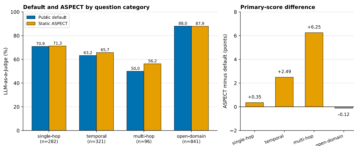
Figure 2. Default and ASPECT by question category. ASPECT's largest descriptive movement is on the 96 multi-hop questions (+6.25 points), followed by temporal (+2.49); open-domain moves -0.12. These stratum differences are descriptive. The registered overall paired comparison is 46 gains to 32 losses, two-sided p=.1405 .
