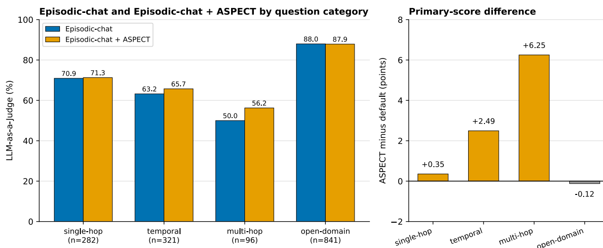
Figure 2. Episodic-chat and Episodic-chat + ASPECT by question category. ASPECT's largest descriptive movement is on the 96 multi-hop questions (+6.25 points), followed by temporal (+2.49); open-domain moves -0.12 . These stratum differences are descriptive. The registered overall paired comparison is 46 gains to 32 losses, two-sided p=.1405 .
