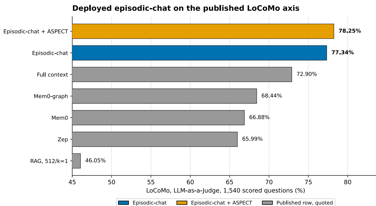
Figure 1. The deployed library on the published LoCoMo axis. Episodic-chat + ASPECT scores 78.25% and Episodic-chat 77.34% on the same 1,540 questions and harness. Grey bars are quoted from arXiv:2504.19413 Table 2 and were not re-run; no paired test is computed against them. Sources: the two committed HH-003 judgement populations and COMPETITIVE_LANDSCAPE.md.
