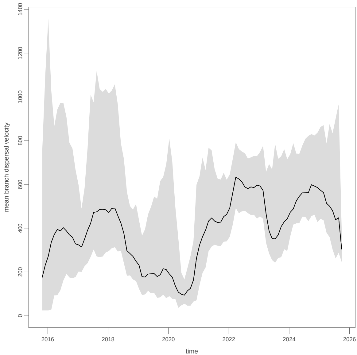
Evolution of mean branch dispersal velocity
