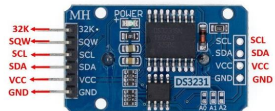
Figura 4 RTC / EEPROM
