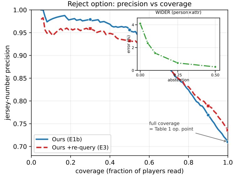
Fig. S11: Reject option, referenced from §5.4 of the main paper: jersey precision vs. coverage (rank by jersey_conf , abstain on the least-confident; precision is over scored digit reads, not the any-OCR precision of Table 1 of the main paper—definitions in Sec. 7, operating points in Tab. S6). E1b solid, re-query E3 dashed; inset: same mechanism on WIDER.
