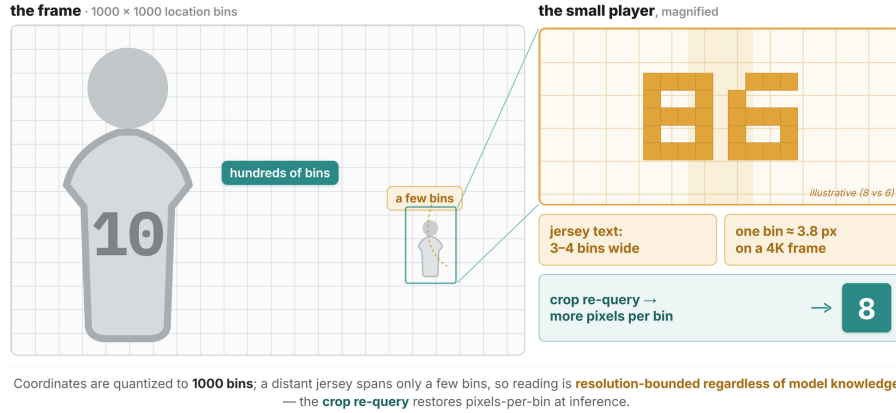
Fig. S4: Quantization, not knowledge, bounds small-text reading. Coordinates are quantized to 1000 location bins, so on a 4K frame one bin is \approx 3.8 px and a distant jersey spans only 3–4 bins—reading is resolution-bounded regardless of model knowledge, and the crop re-query restores pixels-per-bin at inference time. The exact digits in the magnified panels are illustrative only (the “86”/“8” tiles depict the low-resolution ambiguity—e.g. “8” vs. “6”—not a specific ground-truth number).
