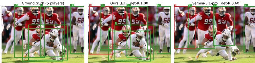
Fig. S12: Qualitative comparison on a crowded frame, referenced from §5.1 of the main paper (ground truth | ours with crop re-query | Gemini-3.1-pro). Box colours: green = prediction matched to a ground-truth player, red = unmatched prediction; box tags are the read jersey numbers. On this frame our detector localizes and reads the small, occluded athletes the API drops (detection recall 1.0 vs. 0.6); the size effect is analyzed in §5.2 of the main paper.
