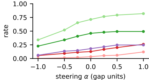
Qwen2.5-7B
