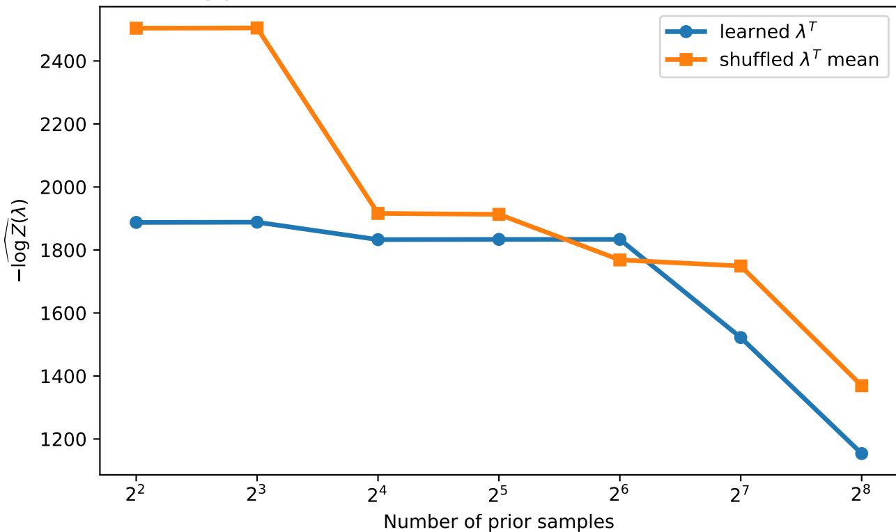
Log-partition estimate: learned vs. shuffled dual variables
