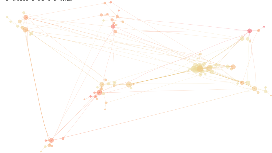
b) Density increased D=0.0301 C=0.370 G=0.725
