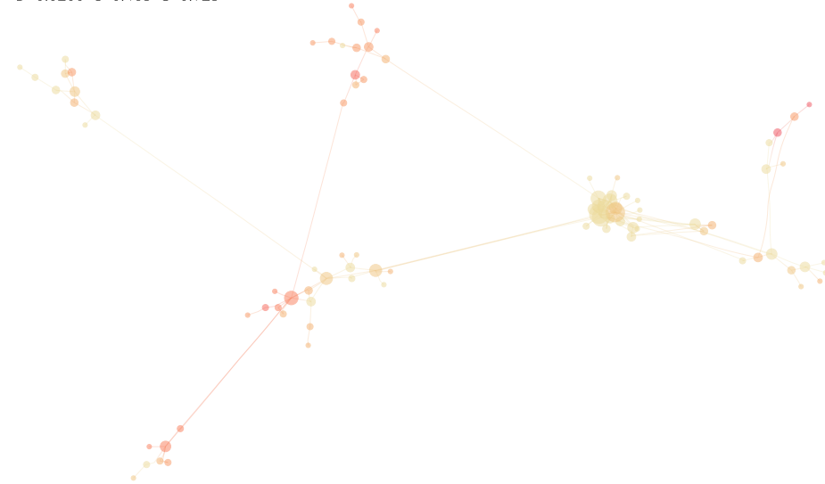
d) Clustering increased D=0.0200 C=0.465 G=0.725
