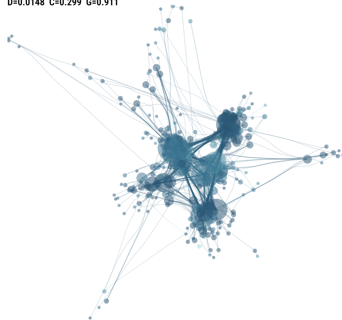
f) Degree Gini increased D=0.0148 C=0.299 G=0.911
