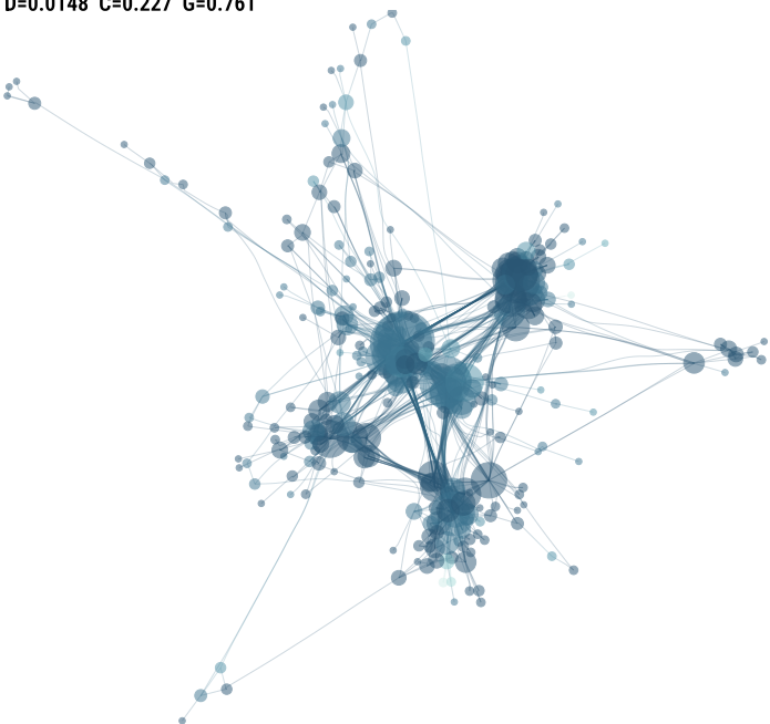
e) Clustering decreased D=0.0148 C=0.227 G=0.761
