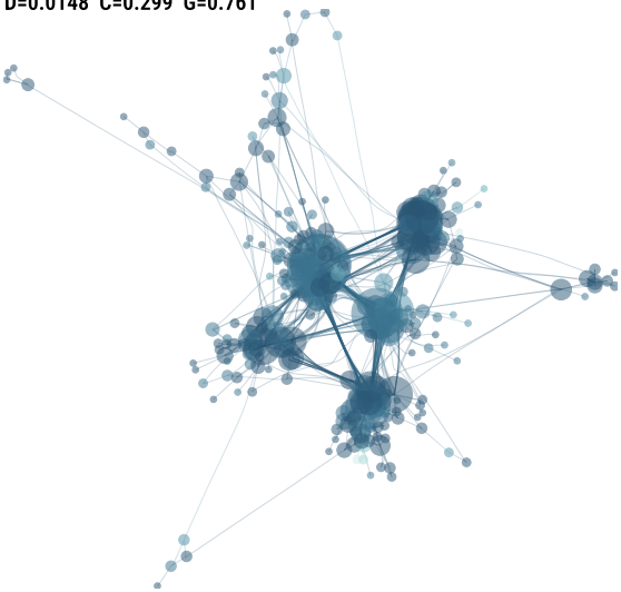
a) Tobacco original D=0.0148 C=0.299 G=0.761
