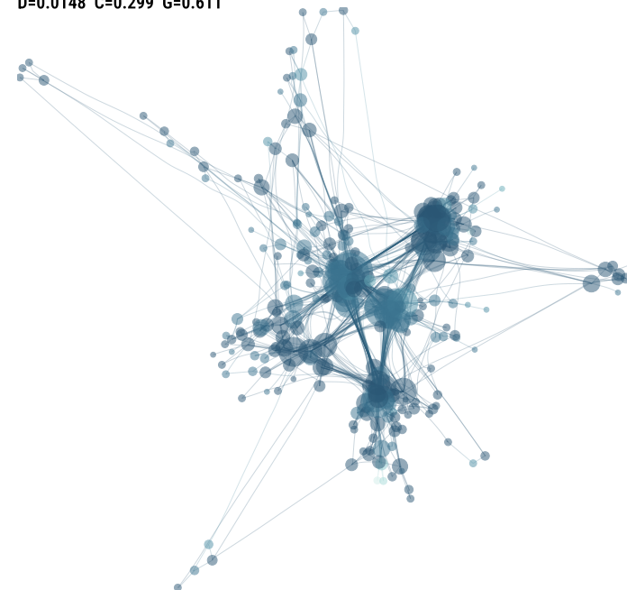
g) Degree Gini decreased D=0.0148 C=0.299 G=0.611
