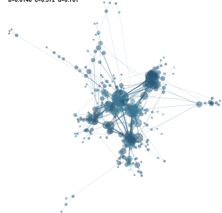
d) Clustering increased D=0.0148 C=0.372 G=0.761
