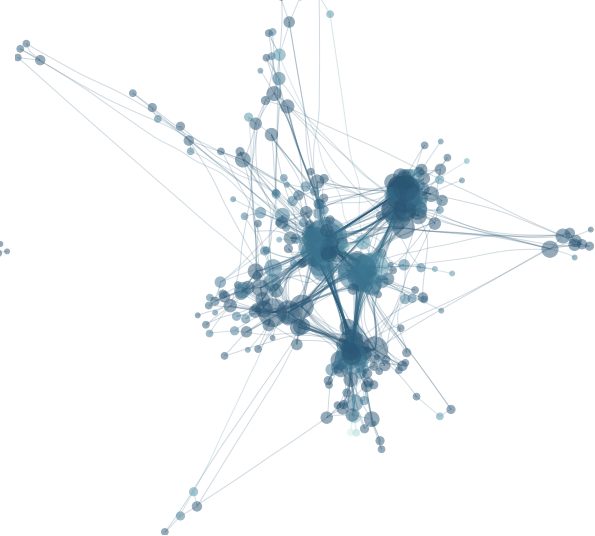
g) Degree Gini decreased D=0.0148 C=0.299 G=0.611
