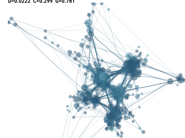
b) Density increased D=0.0222 C=0.299 G=0.761
