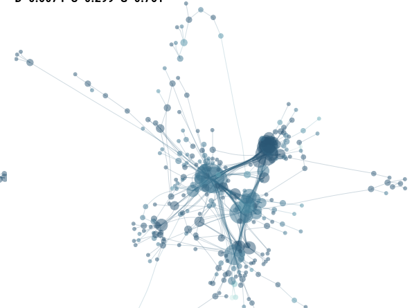
c) Density decreased D=0.0074 C=0.299 G=0.761
