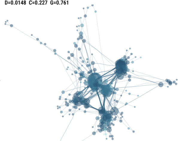
e) Clustering decreased D=0.0148 C=0.227 G=0.761
