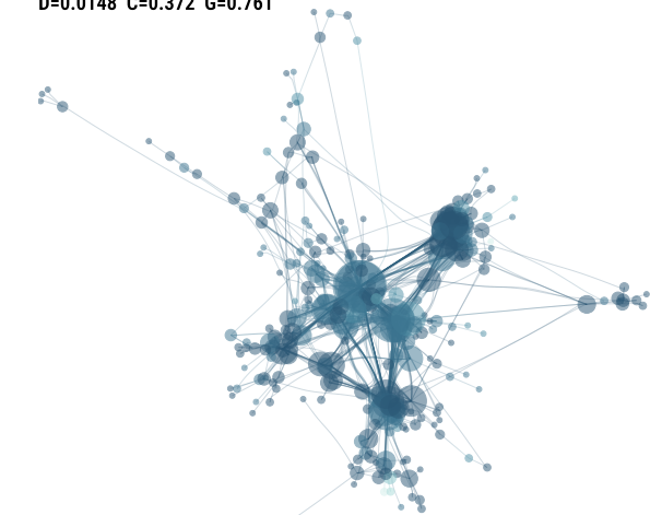
d) Clustering increased D=0.0148 C=0.372 G=0.761
