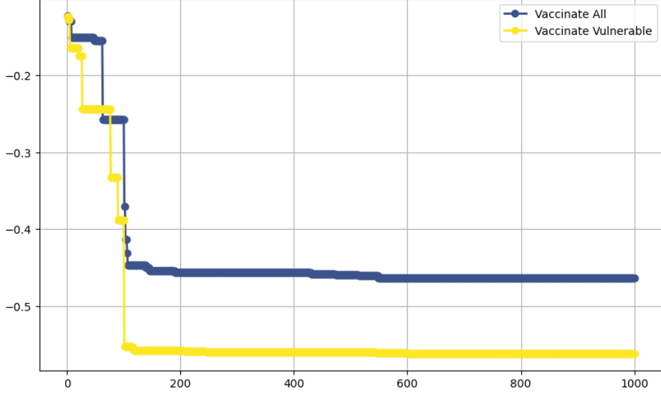
Figure 5: Dynamics of maximisation of total deaths [200-run averages], x -axis: run number, y -axis: population decrease. Approximate maxima are obtained within the first 175 parameter settings. Universal vaccination (blue) caused at most 47% agents to die, for selective vaccination the maximum was 56%.
