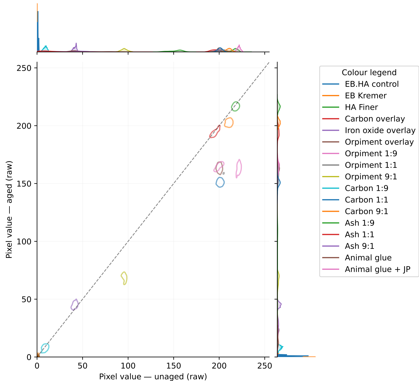
VIL luminescence — all swatches, per-swatch colour (Z-score filtered ; diagonal = no change after ageing)
