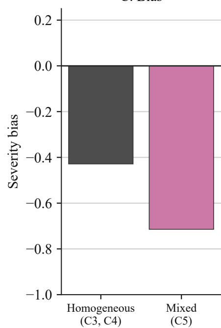
C. Bias
