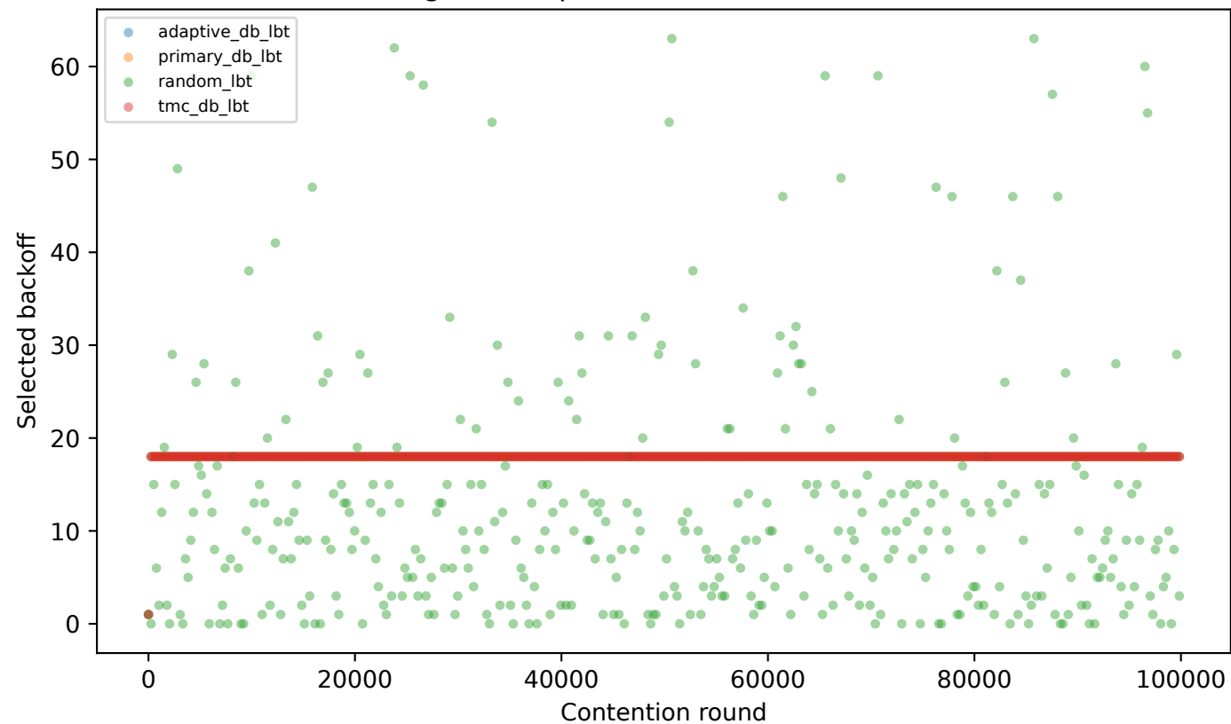
Backoff convergence (reproduction, trace-static-4x4, seed 410)
