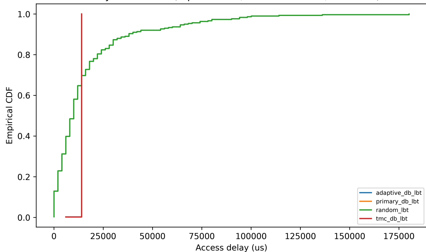
Delay distribution (reproduction, trace-static-4x4, seed 410)
